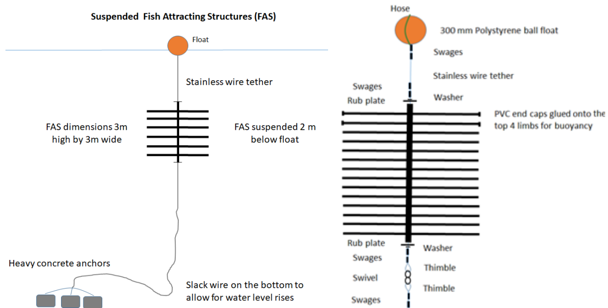
Figure 11 Suspended FAS design
