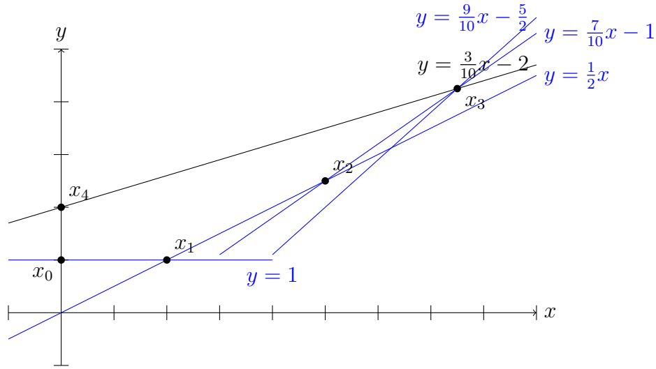
Figure 2: Feasible region of the linear program in Example 2.1.3
