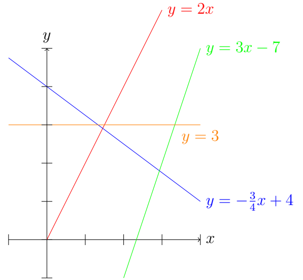
Figure 5: Equations on the x-y plane with y \geq 3 .
