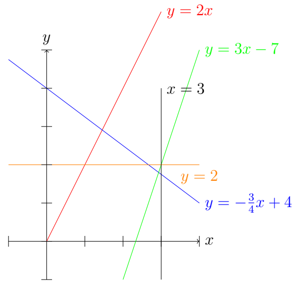
Figure 8: Bound with x \geq 3
