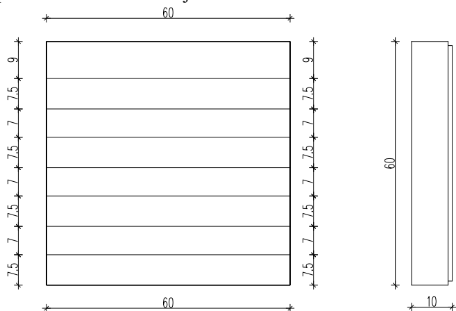
Sl. 7. Prakticni model M3
