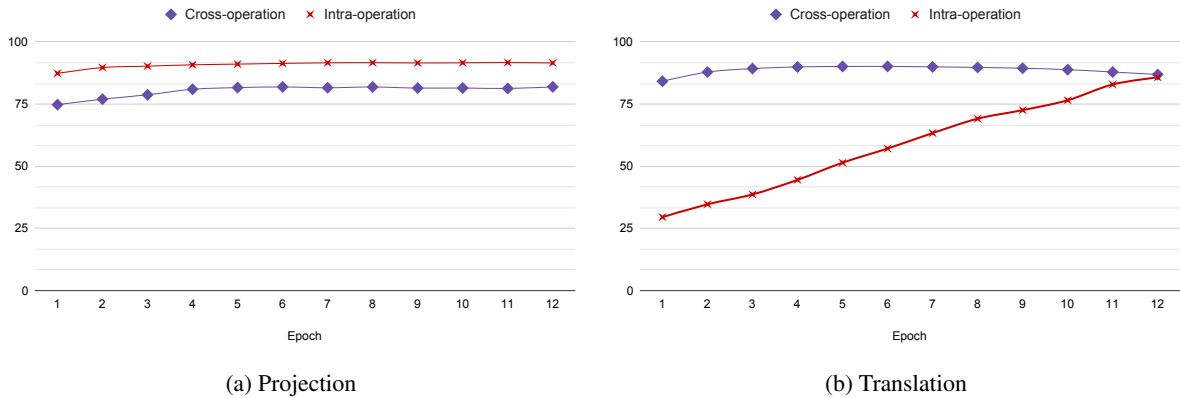
Figure 3: Typical training dynamics of different multi-operational paradigms (MAP on the dev set).
