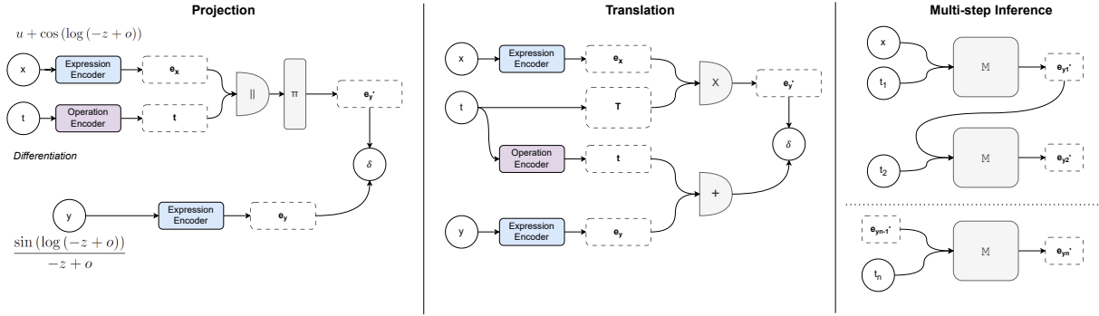
Figure 2: Overview of the joint-embedding predictive architectures for latent multi-operational derivation (left). Schematic workflow for the multi-step propagation of latent operations (right).
