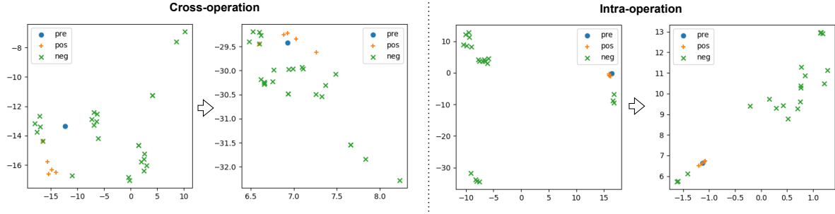
Figure 4: 2D projection of the latent space before and after an operation-aware transformation. The visualization supports the crucial role of the multi-operational paradigm for cross-operational inference, showing, at the same time, that intra-operational inference concerns larger regions and can be achieved in the original expression encoder.
