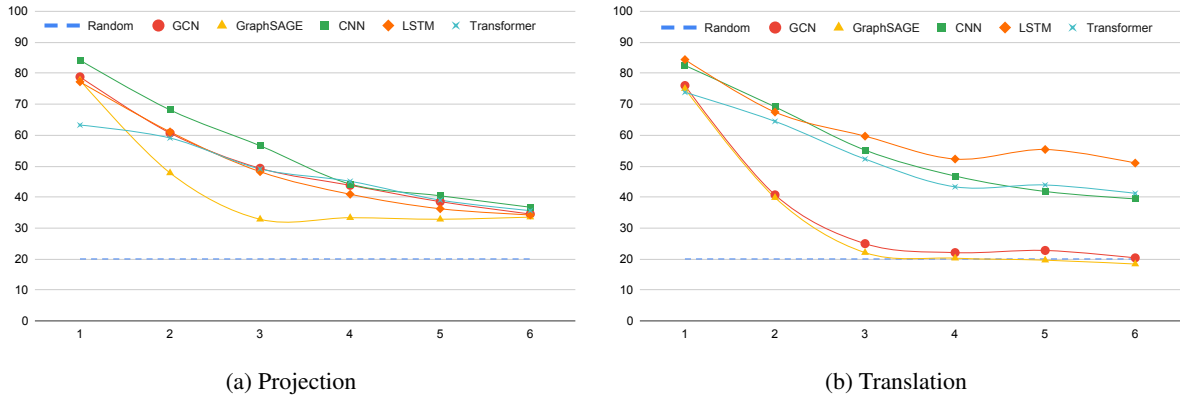
Figure 5: Multi-step derivations in latent space with different multi-operational paradigms and neural encoders.
