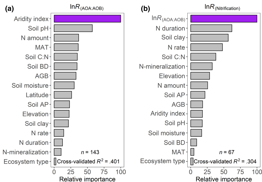
FIGURE 1 The most important predictors for the effects of N loading on AOA:AOB ( \ln R_{(\text{AOA:AOB})} ) and potential nitrification ( \ln R_{(\text{Nitrification})} ). (a) Relative importance of 17 predictors (N form was dropped due to negative importance) of \ln R_{(\text{AOA:AOB})} derived from meta-forest model. (b) Relative importance of 18 predictors (N form and latitude were dropped due to negative importance) of \ln R_{(\text{Nitrification})} derived from meta-forest model. AGB, aboveground biomass; AOA, ammonia-oxidizing archaea; AOB, ammonia-oxidizing bacteria; AP, available phosphorus; BD, bulk density; C:N, the ratio of carbon to nitrogen; MAT, mean annual temperature.
