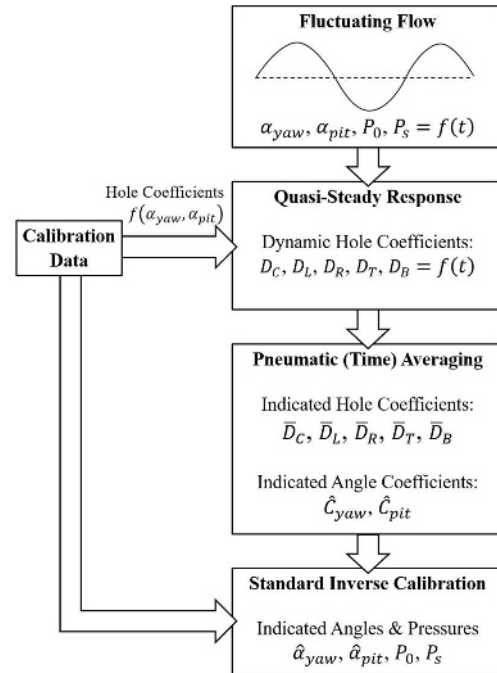
Fig. 2. Quasi-steady model
