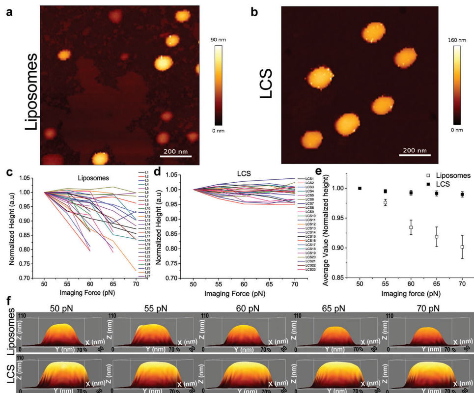
Figure 2. Characterization of nanoparticle mechanical properties by AFM. An overview of the topographic image using an imaging force of 50 pN of a) liposomes and b) the liposome-coated silica (LCS). c–e) Characterization of the height of liposomes (c) and liposome-coated silica (d) as a function of the imaging force. The normalized height data of panel (c) represent the population of liposomes that i) remained in place for at least the three consecutive imaging forces of 50, 55, and 60 pN and ii) did not collapse on the surface. The LCS particles instead (d) could be imaged at all imaging forces (50–70 pN). An overall decrease in the height data was observed in the liposomes (c), whereas the LCS particles (d) hardly deformed with an increase in the imaging force. Panels (c) and (d) show the results for individual particles ( N = 27 and 23 , respectively), while panel (e) shows their average and standard error of the mean. f) 3D topographic images of particles at different imaging forces, showing the deformation of the liposomes with an increase in imaging force in comparison to LCS.
