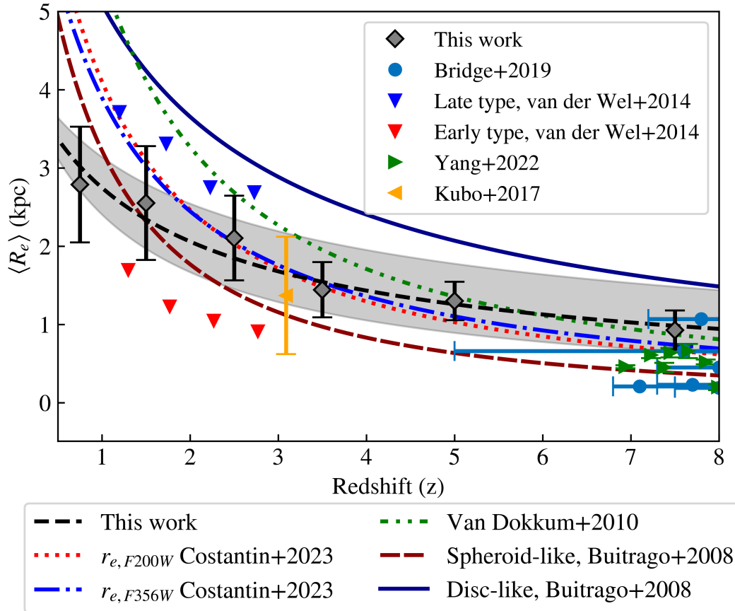
Figure 6. Power law fit showing the size evolution of all galaxies within our sample, compared to results from previous work. The black dashed line is of the form R_e(kpc) = 4.50 \pm 1.32(1+z)^{-0.71 \pm 0.19} , with the grey, shaded area showing the error on the power-law fit. The grey diamond points are the median galaxy sizes in each redshift bin, and error bars are 1\sigma in length. The previous work shown in the Figure uses HST data, except for Yang et al. (2022), which uses JWST data, van Dokkum et al. (2010) which uses NOAO/YaleNEWFIRM Medium Band Survey Data, and Costantin et al. (2023) which uses the TNG50 simulation to produce mock CEERS observations. We note that we only plot redshift errors for Bridge et al. (2019), as radius errors are not provided.
