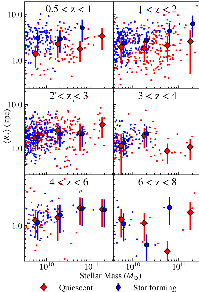
Figure 9. The size-stellar mass distribution of ‘passive’ and ‘star forming’ galaxies, relative to the midpoint of the specific star formation rate in each bin, as explained in subsection 6.2. The larger points represent the median values in mass bins. We use a 50% error floor, with error bars one standard deviation in length, or representing a 50% error on the median, in cases where the error floor is larger.
