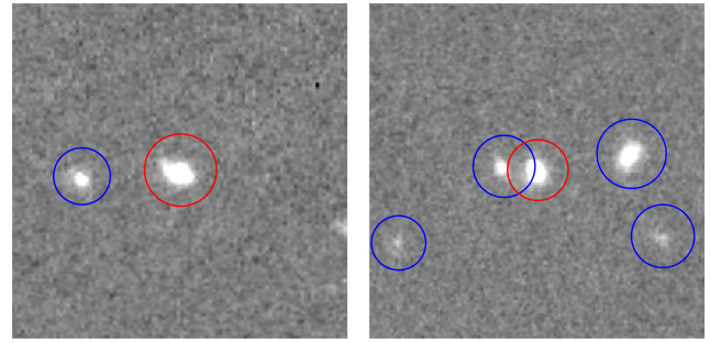
Figure 3. Plots showing the Kron radii (semi-major axis of the Kron ellipse), where the red radius in each image is that of the primary source, and the blue radii are those of the neighbouring sources. We give several scenarios for how these systems would be found. Left: No other sources would be fit simultaneously to the primary, and the pixels belonging to all other objects according to the SExtractor segmentation maps are masked. Right: The source where the Kron radius overlaps that of the primary source are simultaneously fit in this instance, and all other sources would be masked. Cutout sizes shown are 6'' \times 6'' .
