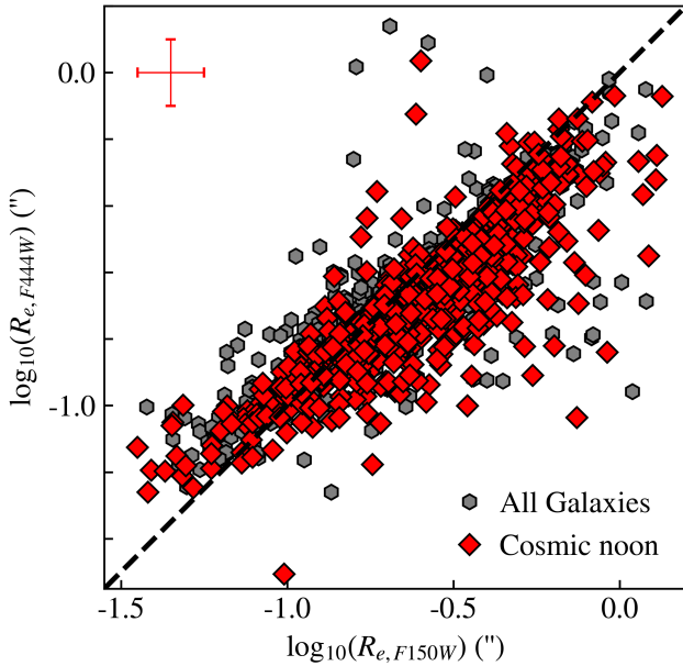
Figure 11. A comparison of sizes measured in the F444W and F150W filters, showing that F444W sizes are smaller than those in F150W. This implies that galaxies measured in the near-infrared with JWST are more compact than rest-frame optical sizes previously measured with HST . Galaxies at cosmic noon ( 1 \leq z \leq 2.5 ) are shown as red diamonds whilst the grey hexagons represent all galaxies within our sample that do not fall within cosmic noon. These latter galaxies do not show the same effect. The black, dashed line is the one-to-one relation. The error bar represents a typical error of 0.2 dex on these measurements.
