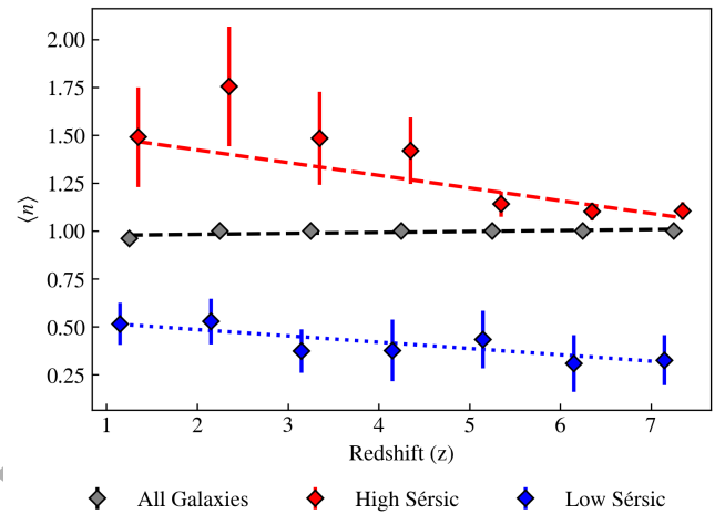
(b) Median Sérsic index of simulated galaxies at each redshift. The lines are the same as explained in the plot of effective radius with redshift (Figure 14a).
