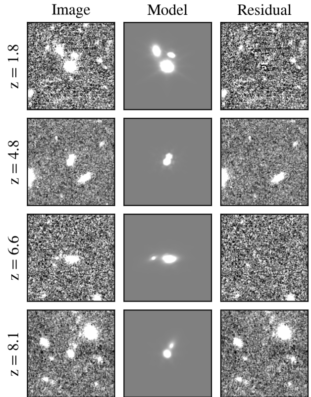
Figure 4. Example fits showing the data image, model image, and the residual image (data - model). Each cutout is 6'' \times 6'' . The redshift of each galaxy is shown to the left of the images.
