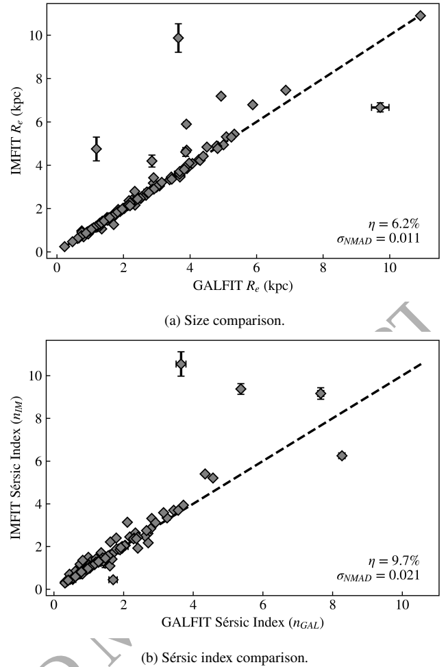
Figure 5. A comparison of two measures - size (top) and Sérsic index (bottom) - as obtained with GALFIT and IMFIT. The black line shows the one-to-one relation. Size and Sérsic index are generally in good agreement, with more variation at larger values, in particular with the Sérsic index. We show the outlier rate ( \eta ) and NMAD in the bottom right corner of each figure.
