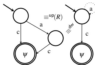
Figure 10: S(\cong^{up}(R), \cong^{dw}) is not GFS for any relation R \subseteq Q \times Q (example adapted from [9]): if we add the dotted transition, the linear tree aac is now accepted. The symbol c has rank 0 and a has rank 1.
