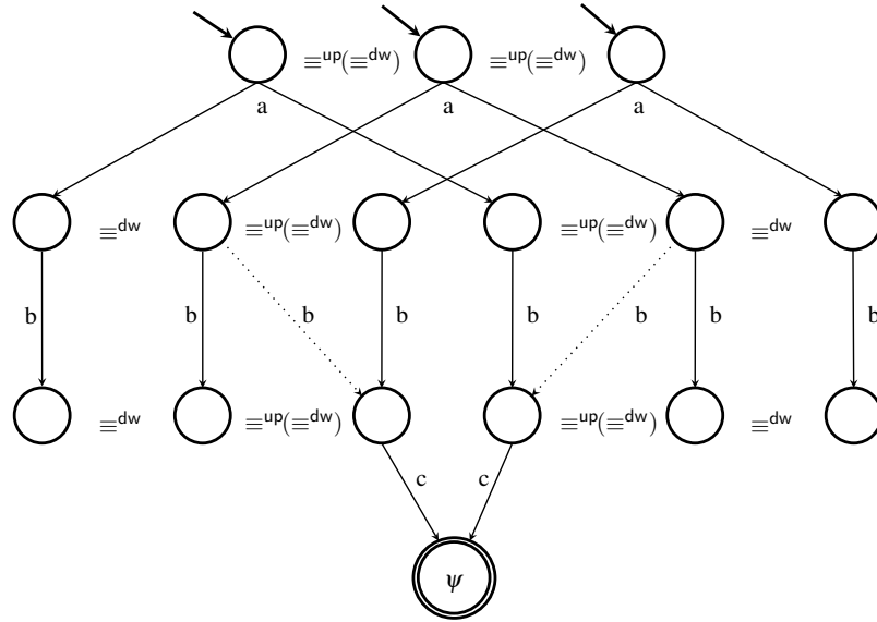
Figure 8: S(id, \cong^{up}(\cong^{dw})) is not GFS: if we add the dotted transitions, the tree a(b(c), b(c)) is now accepted. The symbols c , b and a have ranks 0, 1 and 2, resp.
