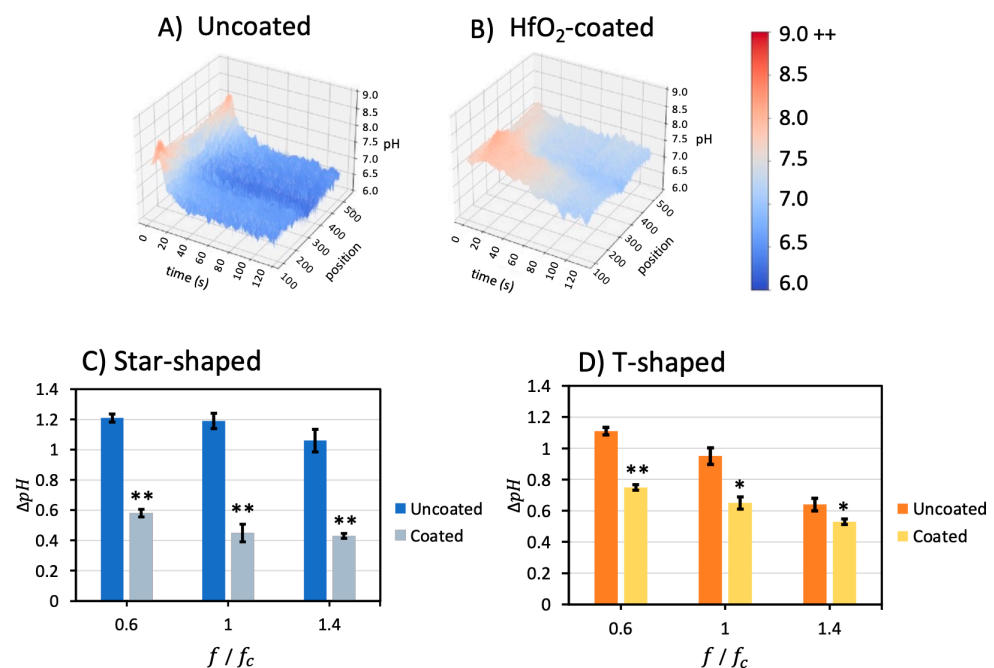
Figure 6. Comparison between uncoated (A) and coated (B) star-shaped devices at 0.6 f_c (1.98 kHz) and 0.07 V_{pp}/\mu\text{m} . The pH decreased from 7.7 to around 6.5 in (A); however, the pH in (B) decreased from 7.7 to around 7.0. Thus, the hafnium oxide layer reduced the Faradaic reaction rate. (C) The \Delta pH for the star-shaped HfO 2 -coated device was reduced by an average of ~60% compared with the uncoated device. (D) The \Delta pH for HfO 2 -coated T-shaped devices was reduced by ~30% on average. Coated/uncoated electrodes were treated as an independent factor in ANOVA; coating has a significant effect on \Delta pH in both geometries at the designated p -values of * p < 0.05 and ** p < 0.001 .
