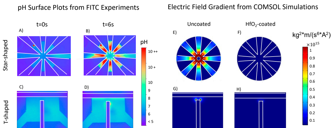
Figure 3. Quantified pH surface plots of star-shaped (A,B) and T-shaped (C,D) uncoated devices at 1.4 f_c and 0.07 V_{pp}/\mu\text{m} . The pH was fairly uniform in both geometry devices around 7.7; pH increased rapidly upon applying an electric field. This burst in pH was much more pronounced in the star-shaped devices. The electric field gradient from COMSOL simulations for uncoated (E,G) and coated (F,H) devices for both geometries. The simulated electric field gradients in both uncoated geometries show similarities in shape with regions of high pH in the respective experiments.
