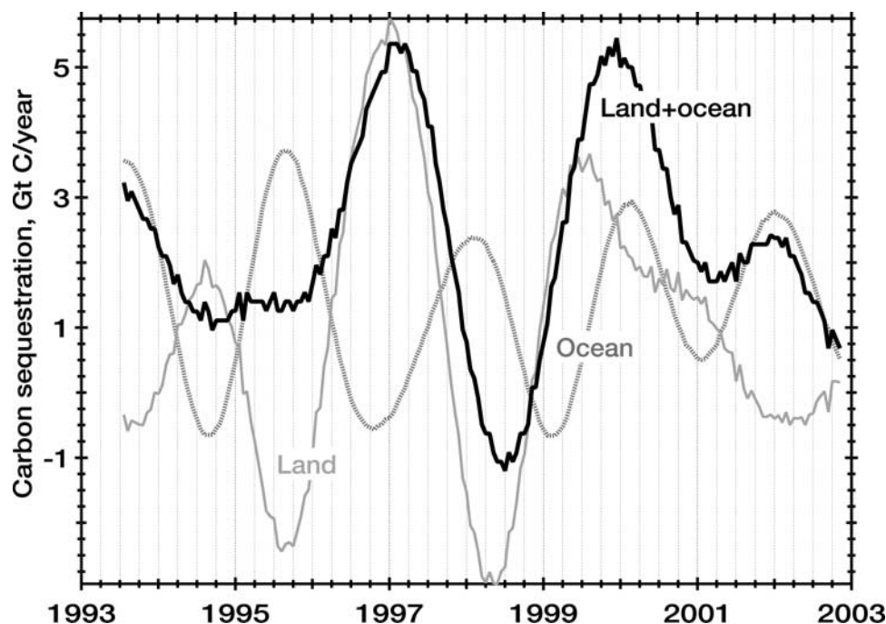
Figure 7. Land and ocean CO 2 sequestration rates calculated from CO 2 and O 2 /N 2 data at CGO, SMO, and BRW. See color version of this figure at back of this issue.
