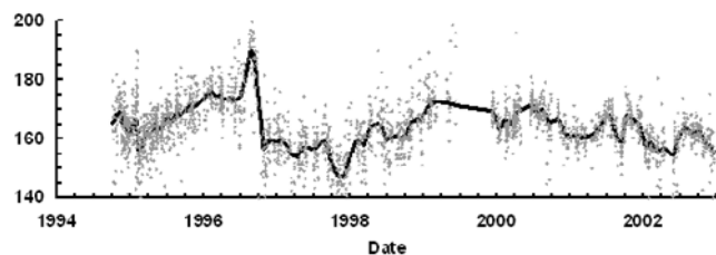
Figure 2. Standard curve, derived solely from the analysis of working standards. Symbols represent individual analyses, while the solid line is the LOESS fit that defines our standard curve.
