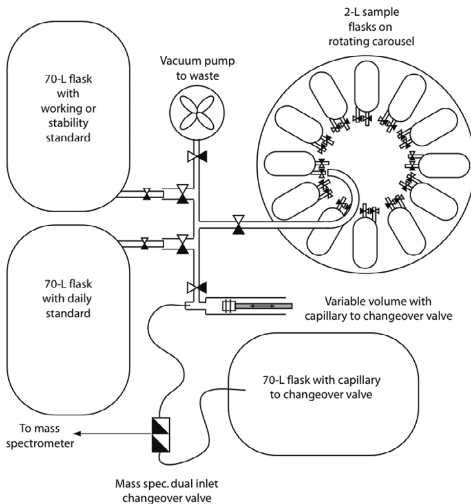
Figure 4. Schematic of the inlet line used at Princeton.
