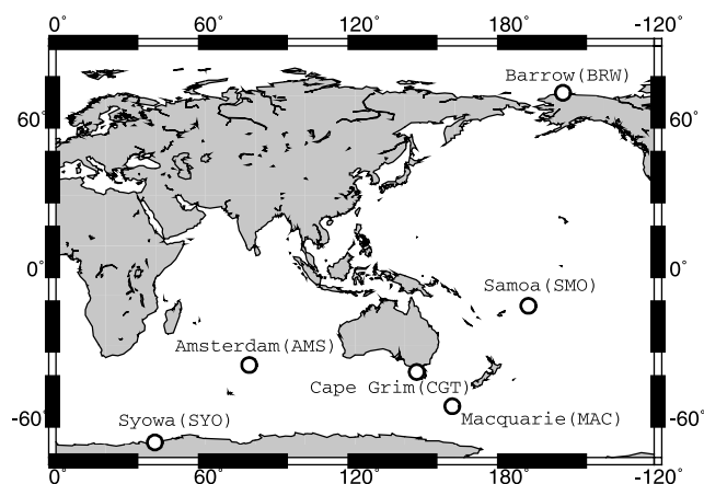
Figure 1. Location of O 2 /N 2 sampling stations.
