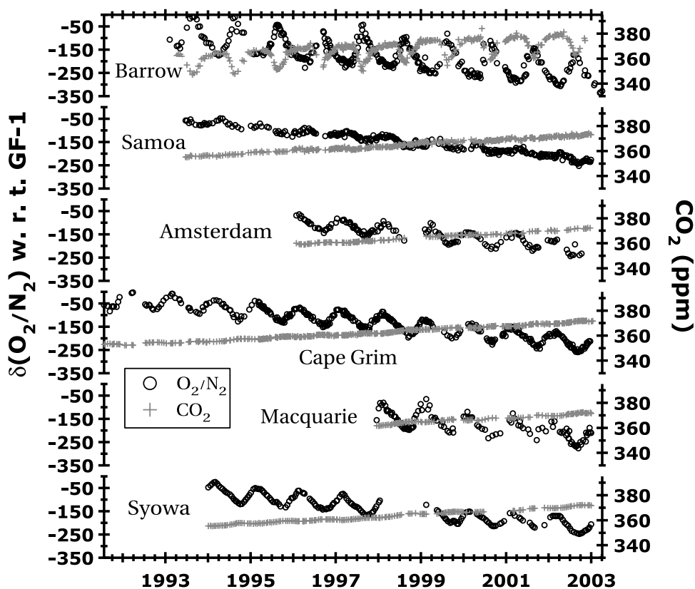
Figure 5. O 2 /N 2 and CO 2 records of this study.
