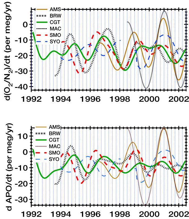
Figure 6. Rates of change of O 2 /N 2 (top) and APO (bottom) in smoothed deseasonalized records from our study sites.
