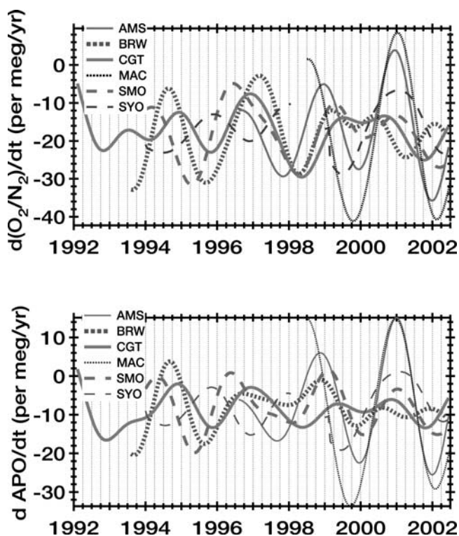
Figure 6. Rates of change of O 2 /N 2 (top) and APO (bottom) in smoothed deseasonalized records from our study sites. See color version of this figure at back of this issue.
