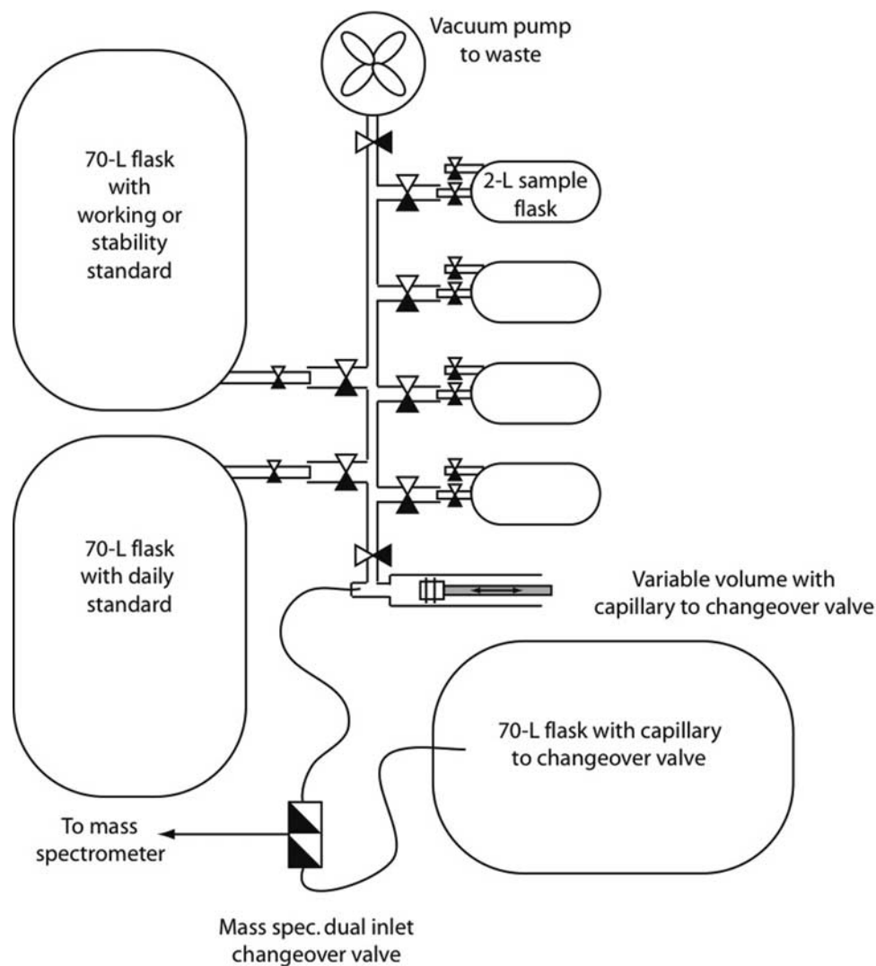
Figure 3. Schematic of the inlet line used at U. R. I. used in the second U. R. I. method.
