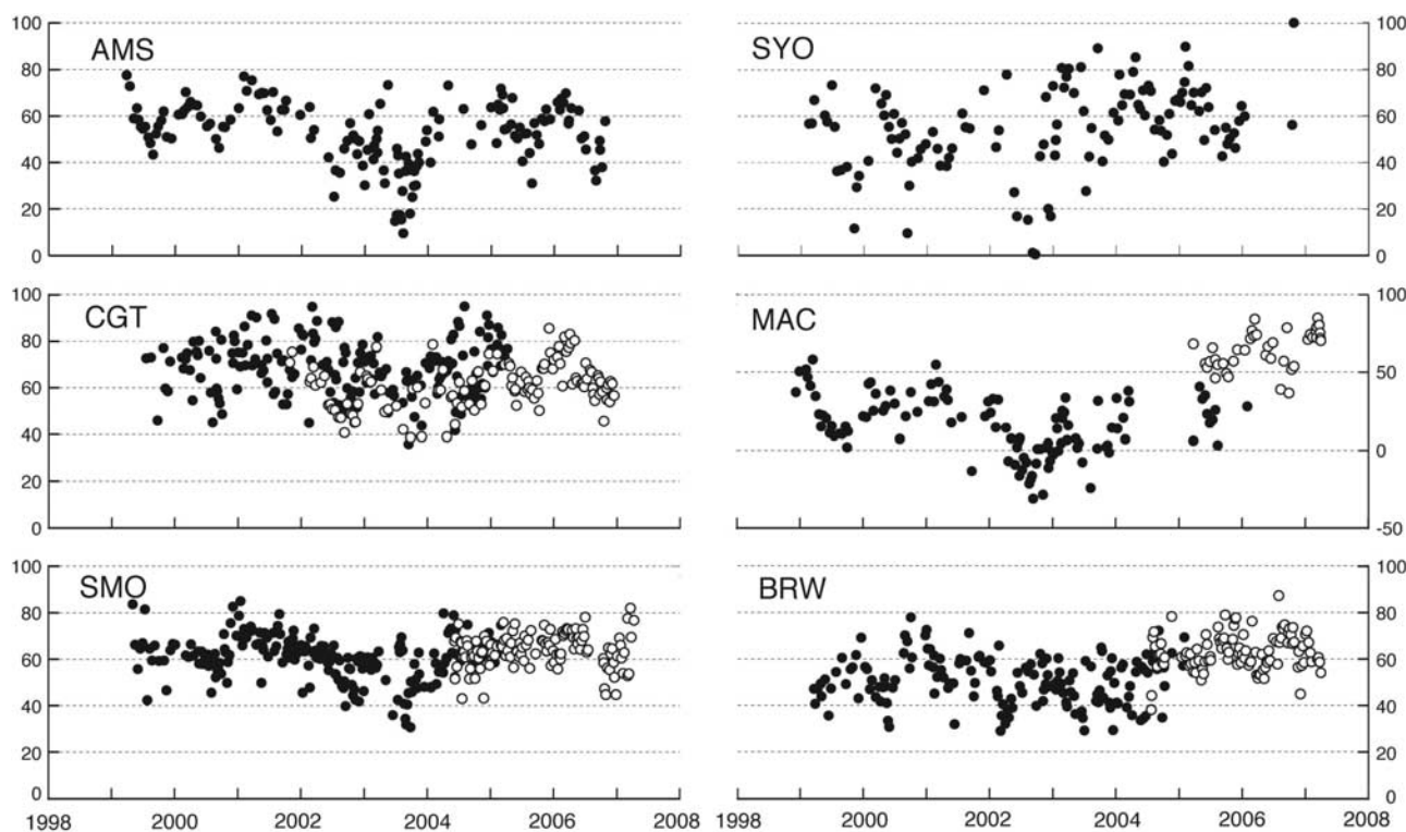
Figure 3. All Ar/N 2 observations (i.e., including outliers) by manual (solid circles) and automated (open circles) sampling at the various stations.
