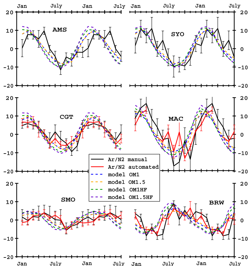
Figure 4. Monthly binned normalized Ar/N 2 climatologies and corresponding atmosphere-ocean model predictions over 1.5 climatological years. For each data set, the annual mean Ar/N 2 is set to zero. The black and red lines are spline fits through manual and automated Ar/N 2 collections, respectively. The vertical bars represent the standard error of the climatological monthly means.
