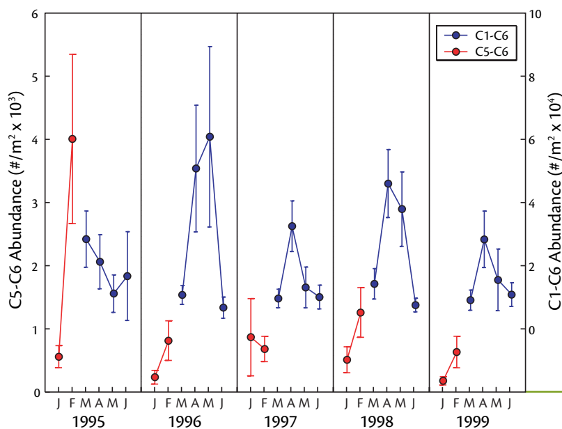
Figure 3. Interannual differences in the mean abundances of C. finmarchicus copepodites observed on Georges Bank from 1995-1999 as determined from the U.S. GLOBEC Northwest Atlantic/Georges Bank Broad-Scale Sampling Program. This broad-scale sampling program included Multiple-Opening Closing Net and Environmental Sensing System tows from approximately 40 stations spread relatively uniformly over Georges Bank and its surrounding waters (McGillicuddy et al., 2001). Copepodite five and six (C5-C6) abundances are shown for January and February in red. These are principally G 0 animals that grew up the previous year and subsequently emerged from diapause. Copepodite one through six (C1-C6) abundances are shown for March through June in blue. These are principally G 1 and G 2 animals that grew up in the specified year. Bars through circles correspond to 95 percent confidence intervals.
