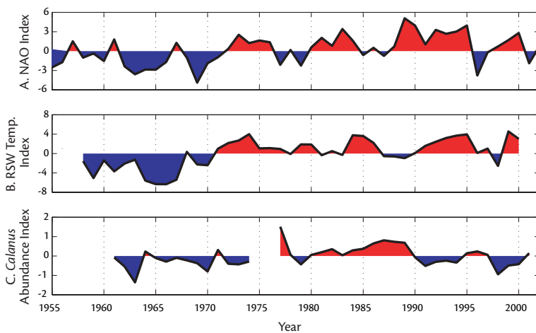
Figure 4. Considerable interannual variability was observed in the time series of A.) the NAO Index, B.) the RSW Temp. Index, and C.) the C. finmarchicus Abundance Index. The NAO Index is the mean difference, expressed as an anomaly from the long-term mean, in atmospheric pressure during winter between the North Atlantic's subtropical high-pressure system, measured in Lisbon, Portugal, and the subpolar low pressure system, measured in Stykkisholmur, Iceland (Hurrell, 1995). The RSW Temp. Index is the dominant mode derived from a principal components analysis of eight slope-water temperature-anomaly time series from the Gulf of Maine and Western Scotian Shelf (MERCINA, 2001). It was introduced as an indicator of the modal state of the CSWS, with positive values of the index corresponding to maximum modal state conditions and negative values corresponding to minimum modal state conditions. The C. finmarchicus Abundance Index is the mean annual abundance anomaly for late copepodites and adults of this species calculated each year as the mean difference between log-transformed observed abundances and log-transformed expected abundances (MERCINA, 2001). It is derived from Continuous Plankton Recorder survey data that have been collected from the Gulf of Maine since 1961 (Jossi and Goulet, 1993).
