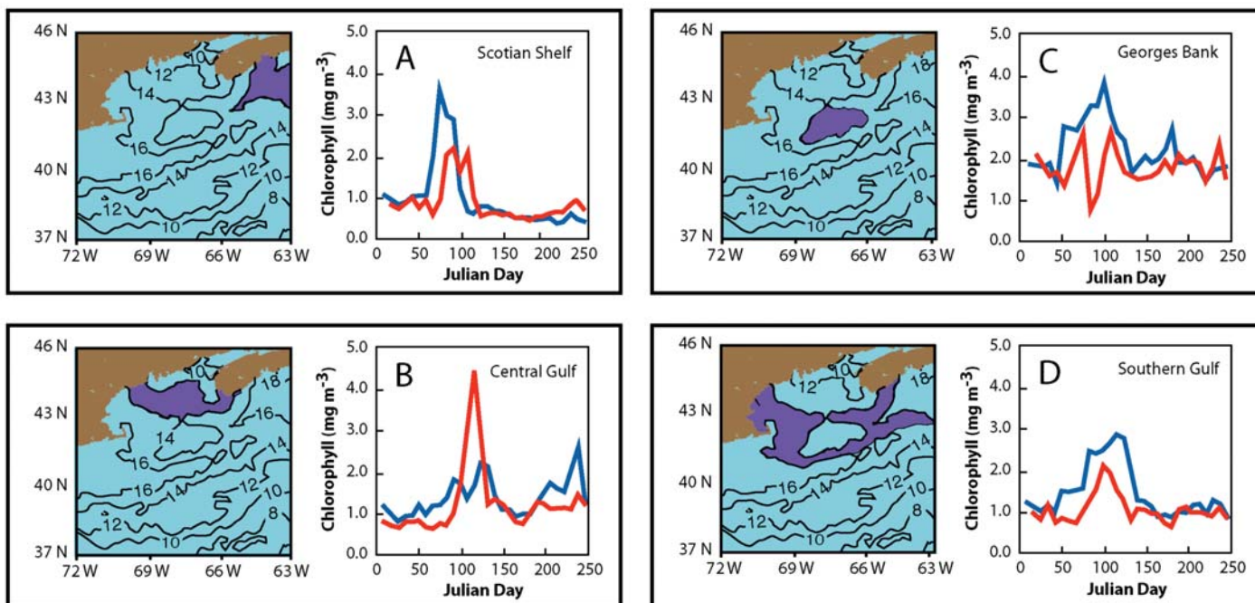
Figure 2. Large interannual differences in the seasonal cycles of chlorophyll concentration were observed during 1998 (red lines) and 1999 (blue lines) in four subregions of the Northwest Atlantic: (A) the southwestern Scotian Shelf, (B) the central Gulf of Maine, (C) Georges Bank, and (D) the southern Gulf of Maine and deep waters adjacent to Georges Bank. For each subregion (shaded on each map in purple), the chlorophyll time series are derived from spatial averages of Sea-viewing Wide Field-of-View Sensor data (SeaWiFS 4th reprocessing data set distributed by NASA's Goddard Space Flight Center Earth Sciences Distributed Active Archive Center). Subregions are based on similarity in the amplitude of seasonal change in sea-surface temperature (SST) as determined from analysis of Advanced Very High-Resolution Radiometer climatology data (AVHRR Pathfinder data set distributed by the NASA Jet Propulsion Laboratory's Physical Oceanography Distributed Active Archive Center). The analysis involves computing the amplitude of seasonal change in SST at each pixel location and then contouring the result at 2-degree intervals. Individual subregions are bound by the 2-degree contour intervals shown on each map.
