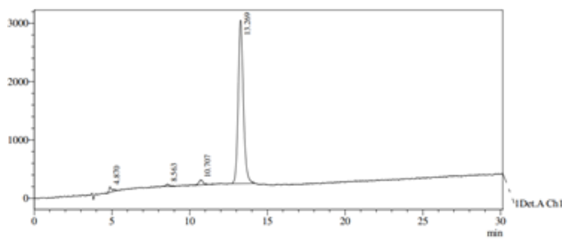
GAMBAR 3. Hasil analisa HPLC brazilin.
