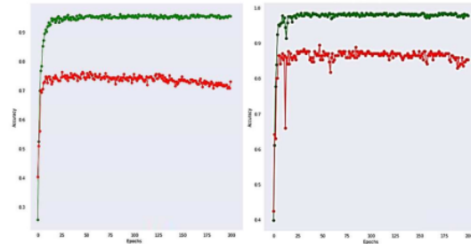
Fig. 8. Training accuracy (green) and validation accuracy (red) of damage location (left) and damage severity (right) classifiers with DCGAN image augmentation.
