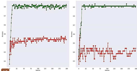
19 Fig. 6. Training accuracy (green) and validation accuracy (red) of damage location (left) and damage severity (right) classifiers without image augmentation.
