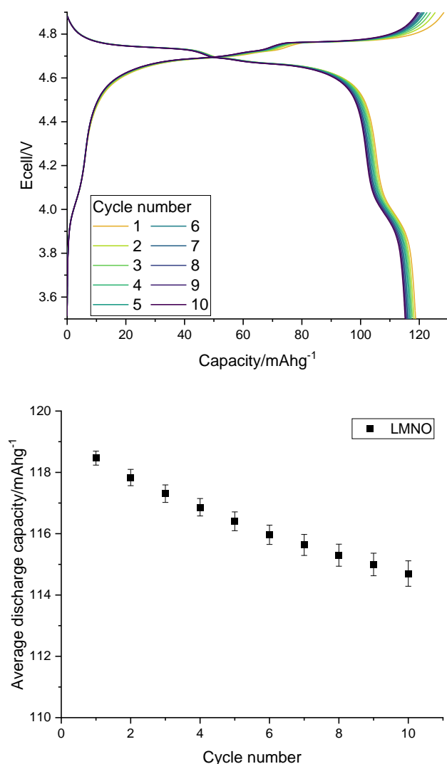
Figure 8: a. Galvanostatic charge-discharge profile (above) and b. average gravimetric discharge capacity against cycle number (below) for LMNO. Cells were cycled at 10 mA g -1 between 3.5-4.9 V.
