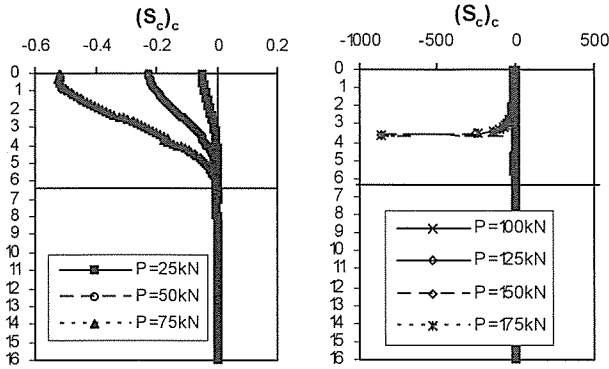
Fig. 17 Distribution of (S_c)_c for 50% clay
