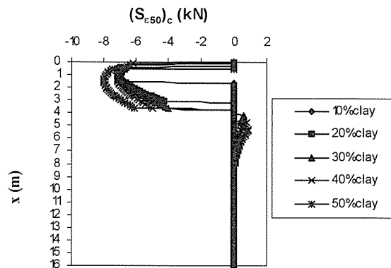
Fig. 34 Effect of clay thickness on (S_{e50})_c for constant deflection criterion
