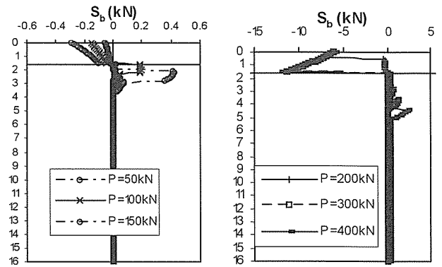
Fig. 18 Distribution of S_b for 10% clay
