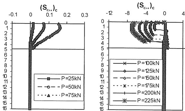
Fig. 5 Distribution of (S_{\epsilon_{50}})_c for 30% clay
