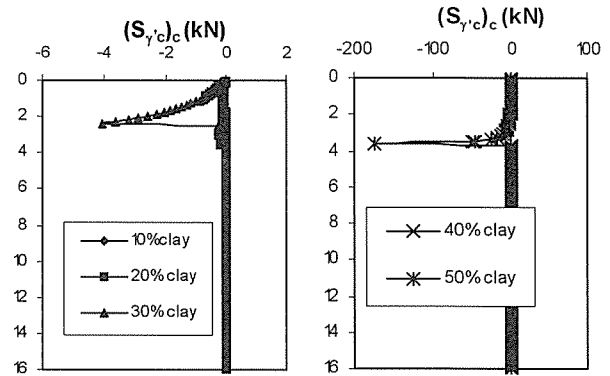
Fig. 30 Effect of clay thickness on (S_{\gamma'c})_c at P=150kN
