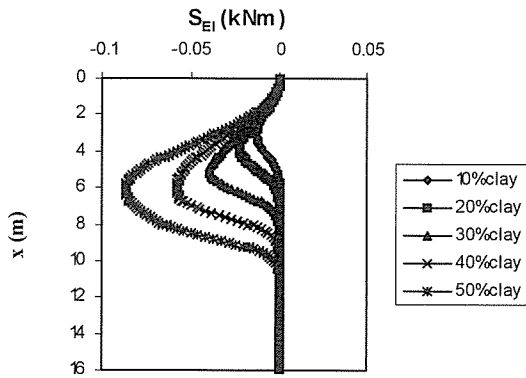
Fig. 33 Effect of clay thickness on S_{EI} at P=150\text{kN}
