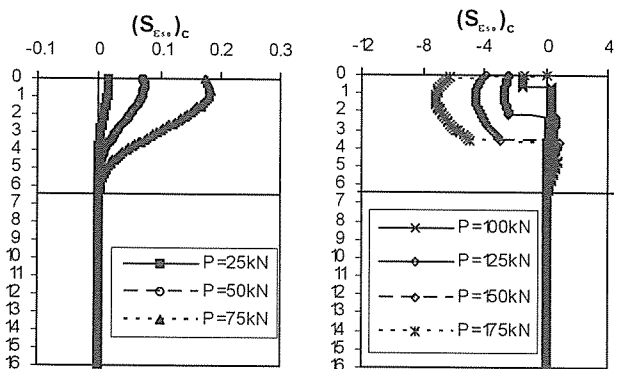
Fig. 6 Distribution of (S_{\epsilon_{50}})_c for 40% clay
