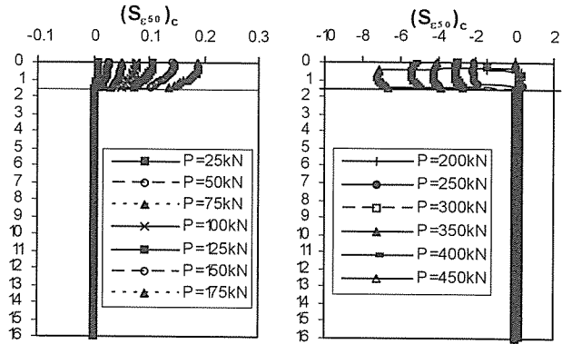
Fig. 3 Distribution of (S_{\epsilon_{50}})_c for 10% clay
