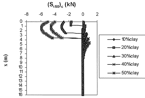
Fig. 29 Effect of clay thickness on (S_{e50})_c at P=150kN
