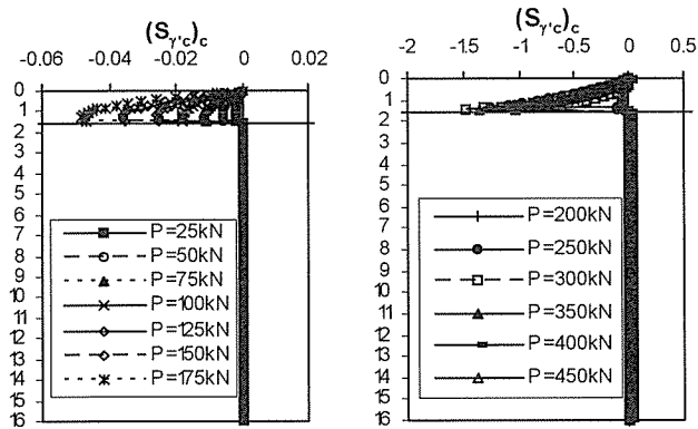
Fig. 8 Distribution of (S_{\gamma'_c})_c for 10% clay
