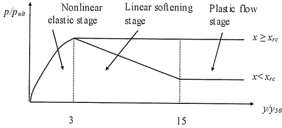
Fig. 2 Nonlinear behavior of soft clay subjected to cyclic loading after Matlock et al. (1970)
