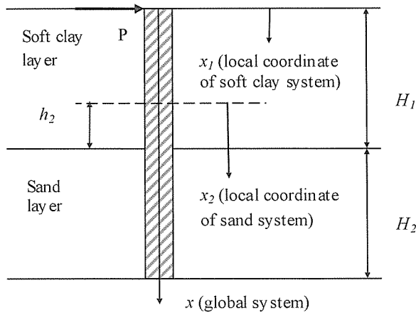
Fig. 1 The coordinate systems of a pile embedded in a non-homogeneous soil
