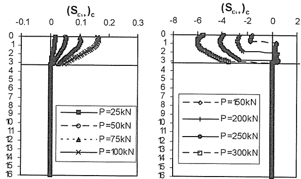
Fig. 4 Distribution of (S_{\epsilon_{50}})_c for 20% clay
