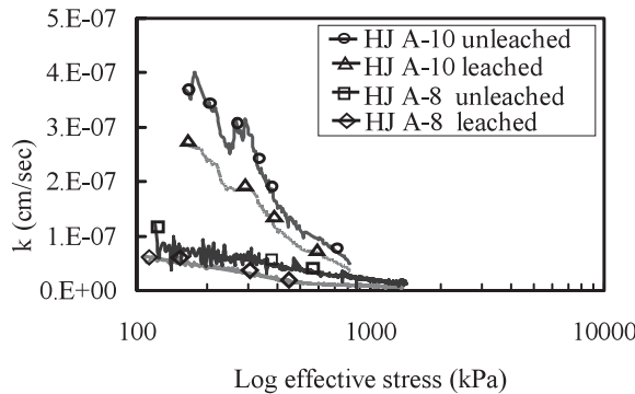
Fig. 11 Hydraulic conductivity compare of leached and unleached specimens
