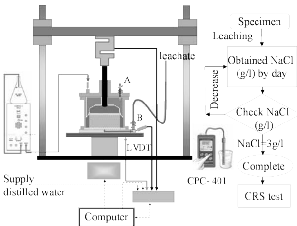
Fig. 3 Schematic diagram of leaching procedure and assembly on the CRS apparatus
