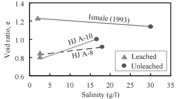
Fig. 5 Void ratio change with salinity at the end of CRS test
