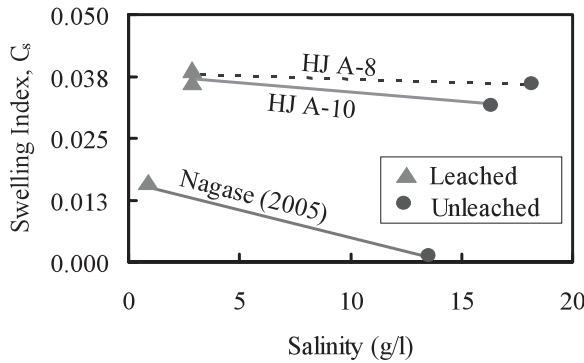
Fig. 10 Variation of swelling index with salinity
