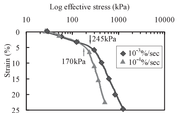
Fig. 8 Strain rate effects on leached specimens
