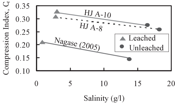
Fig. 9 Variation of compression index with salinity
