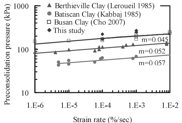
Fig.13 Linear relation between preconsolidation pressure and strain rate
