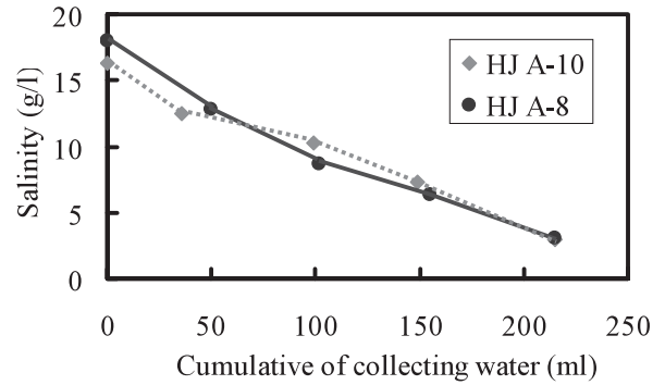
Fig. 4 Variation of soil salinity with the cumulative of collecting water
