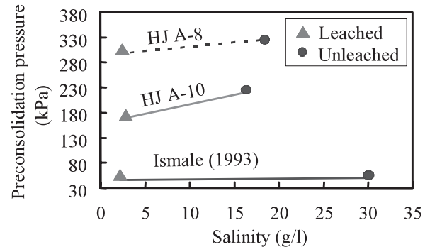
Fig. 12 Variation of preconsolidation pressure with salinity
