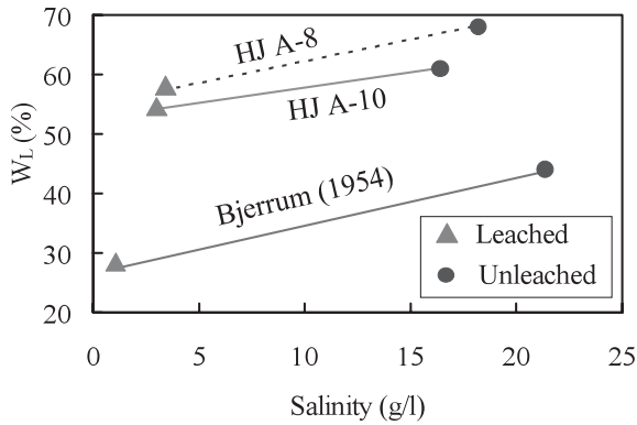
Fig. 6 Variation of liquid limit ( W_L ) with salinity
