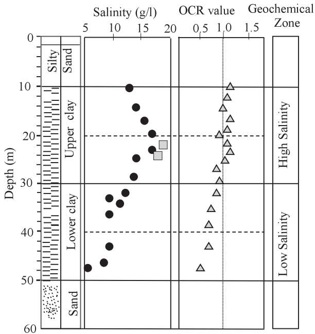
Fig. 2 Soil profile and geo-chemical analysis for clay at BH4, Hwajeon site (Rao 2004)
