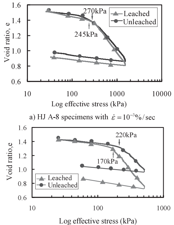
Fig. 7 CRS tests with unleached and leached specimens
