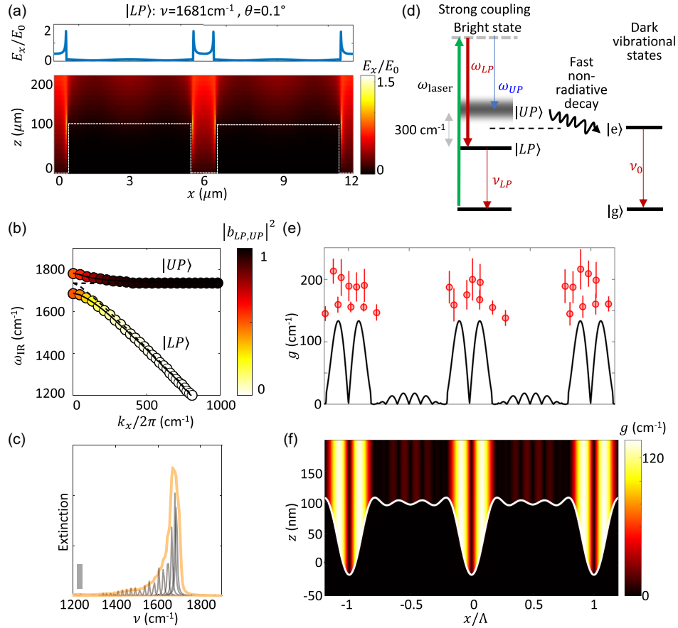
FIG. 4. Polariton-enhanced Raman scattering in gratings. (a) Field distribution ( E_x/E_0 ) for the lower polariton under near-normal incidence ( \theta = 0.1^\circ ) transverse-magnetic (TM) excitation perpendicular to the grating grooves (dashed). Gold permittivity from Ref. [26]. (b) Coupled oscillator fit to RCWA simulations of grating scattering for upper and lower polariton modes vs momentum ( k_x ). Colors show vibrational Hopfield coefficient fraction (Supplemental Material, Sec. S2 [24]). (c) Molecular density-of-states (corrected and angle-averaged) showing asymmetric broadening of LP peak (gray bar indicating extinction of 0.1). (d) Polariton states showing scattering from ground state to bright (strongly coupled) and dark states, labeling Raman scattering ( \omega ) and infrared absorption ( \nu ). (e) Plasmon-vibration coupling strength g vs normalized position x/\Lambda , with red points from Fig. 2. (f) Map of spatial plasmon-vibration coupling strength g along the \Lambda = 4.7 \mu\text{m} grating (modeled surface profile in white).
