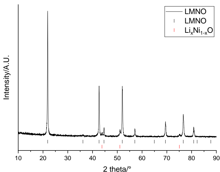
Figure 7: XRD patterns of \text{LiMn}_{1.5}\text{Ni}_{0.5}\text{O}_4 made from recovered LMO (Co \text{K}\alpha ). Tick marks correspond to LMNO (black) and \text{Li}_x\text{Ni}_{1-x}\text{O} (red).
