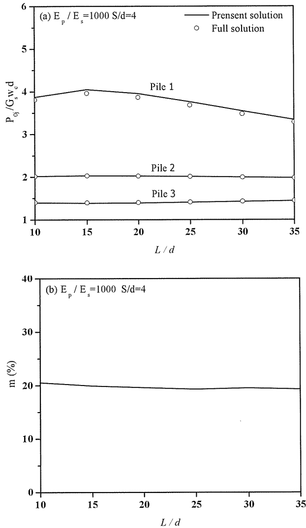
Fig. 8 Comparison of present solution with full solution
