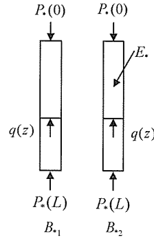
(c) Fictitious piles
