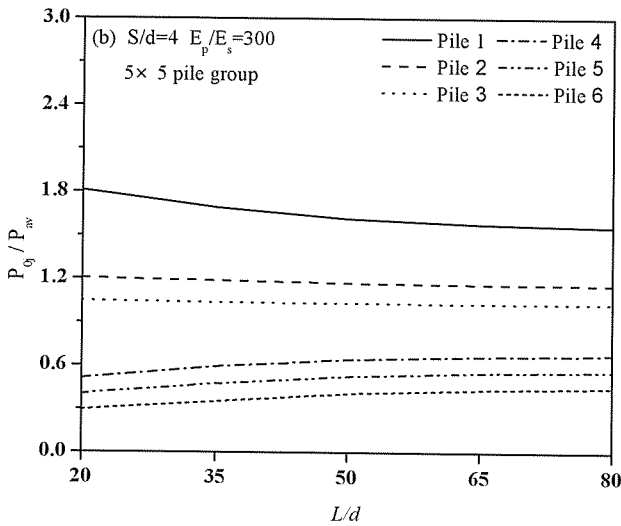
Fig. 7b Load distribution versus pile slenderness ratio
