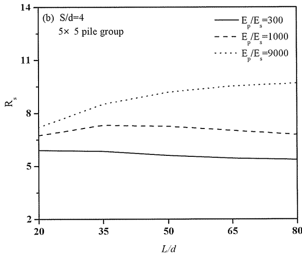
Fig. 5 Pile group settlement ratio versus pile slenderness ratio
