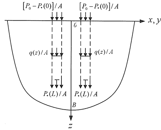
(b) Extended soil
