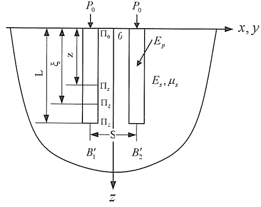
(a) Pile-soil system
