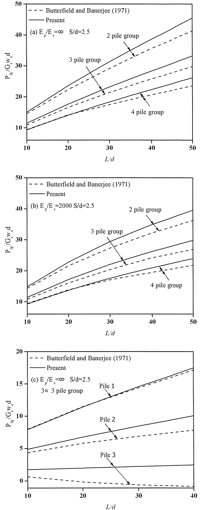
Fig. 3a Comparison of load distributions among individual piles in pile groups
