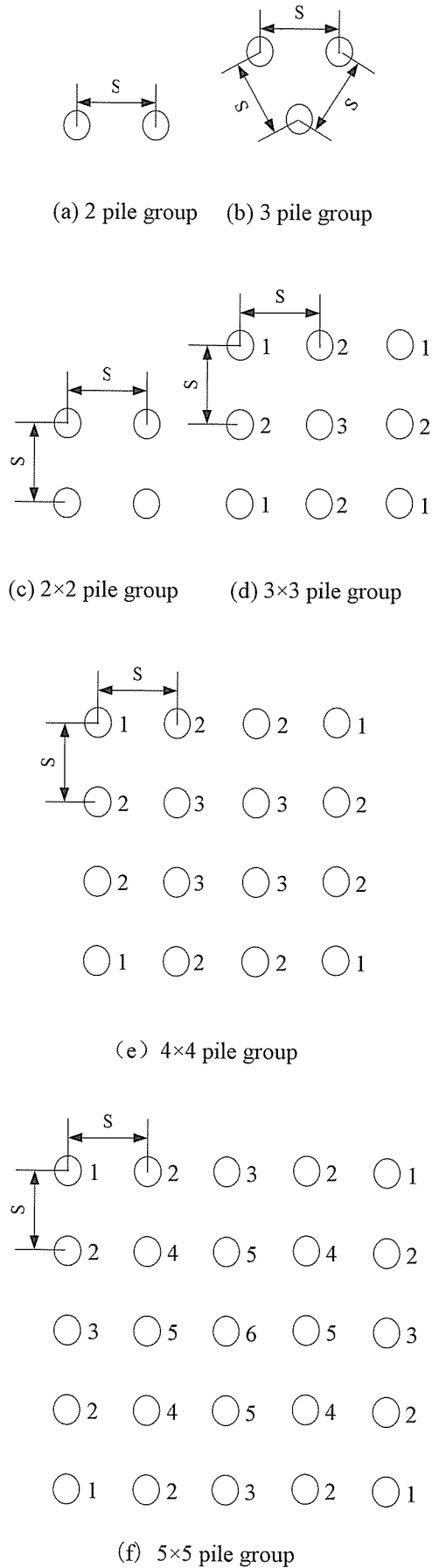
Fig. 2 Configurations for different pile groups
