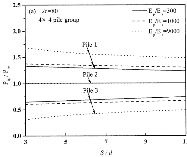
Fig. 6a Load distribution versus pile spacing ratio
