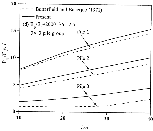
Fig. 3b Comparison of load distributions among individual piles in pile groups
