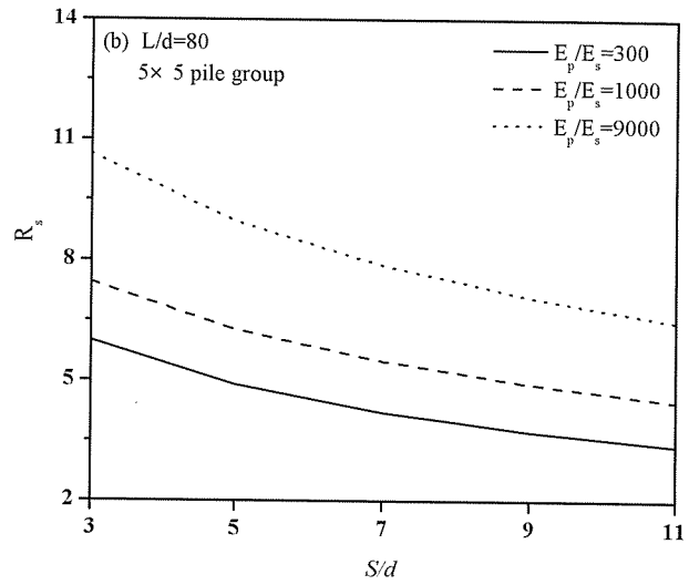
Fig. 4 Pile group settlement ratio versus pile spacing ratio
