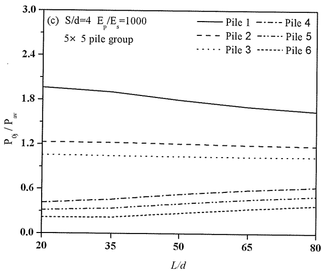
Fig. 7a Load distribution versus pile slenderness ratio
