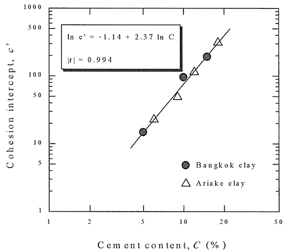
Figure 14: Relationship between cohesion intercept and cement content of induced cemented Bangkok and Ariake clays
