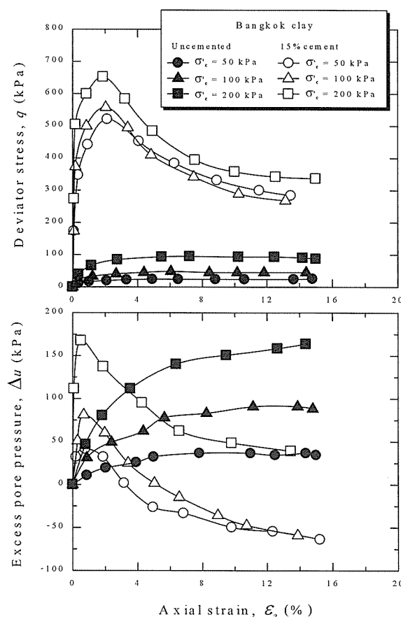
Fig. 5 ( q, \epsilon_a ) and ( \Delta u, \epsilon_a ) of induced cemented Bangkok clay at pre-yield state and at cement content of 15%
