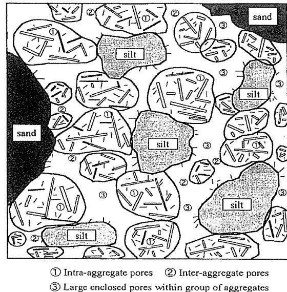
Fig. 1 Structure of clay (Nagaraj et al., 1990)
