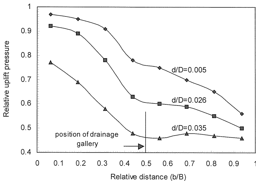
Fig. 2 Relative uplift pressure ( P/H_1 ) versus relative distance (b/B) for different values of the relative diameter ( d/D ) ( H_2/H_1 = 0.39 , h/D = 0.0 & L/D = 0.39 )
