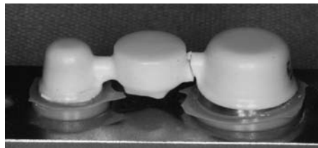
Fig. 4 The observation shows the typical fractured framework under static load bearing test.
