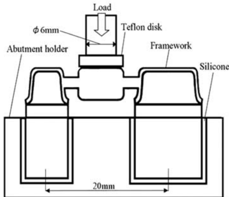
Fig. 2 Test device for determination of static load bearing of 3-unit framework
