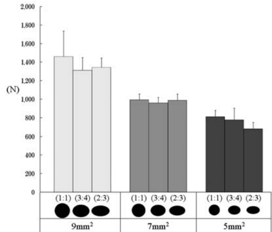
Fig. 3 Load required for fracture by type of connector
