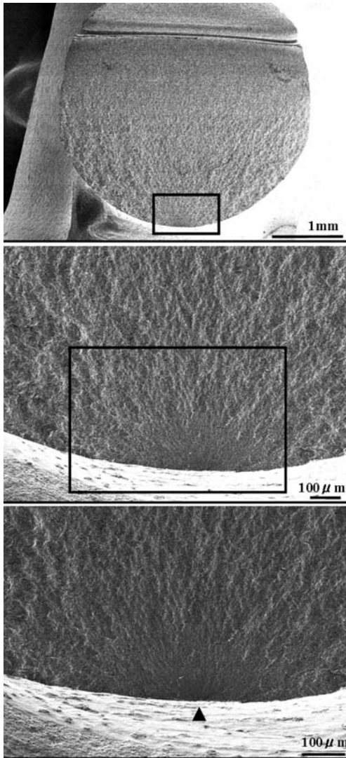
Fig. 5 SEM observation showed cross-section of fracture.
