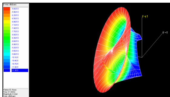
Gambar 10. Radiation Pattern
