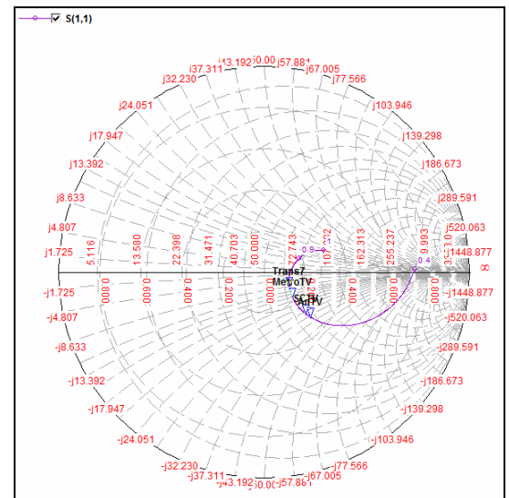
Gambar 12. Smith Chart
