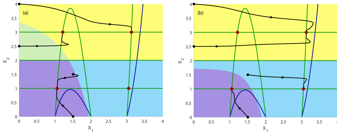
Figure 9. Time evolution of the non-autonomous system shown in Eq. (8) with decreasing impact of the driver c in the interval [0.4, 0.1] together with four exemplary trajectories (timescale separation between system 1 and 2 \varepsilon = 0.1 ): (a) fast rate with 0 \leq t \leq 2.0 , v = -0.15 and T_r = 2.0 and (b) slow rate with 0 \leq t \leq 8.0 , v = -0.0375 and T_r = 8.0 . Attractors are indicated by filled dark-red circles. Dark-blue curves: nullclines at the beginning of the parameter drift at t = 0 and c = 0.4 ; dark-green curves: nullclines at the end of the parameter drift at t = T_{end} = 200 and c = 0.1 . The non-autonomous basins of attraction are presented at the end of the simulation T_{end} in light green, yellow, violet and light blue.
