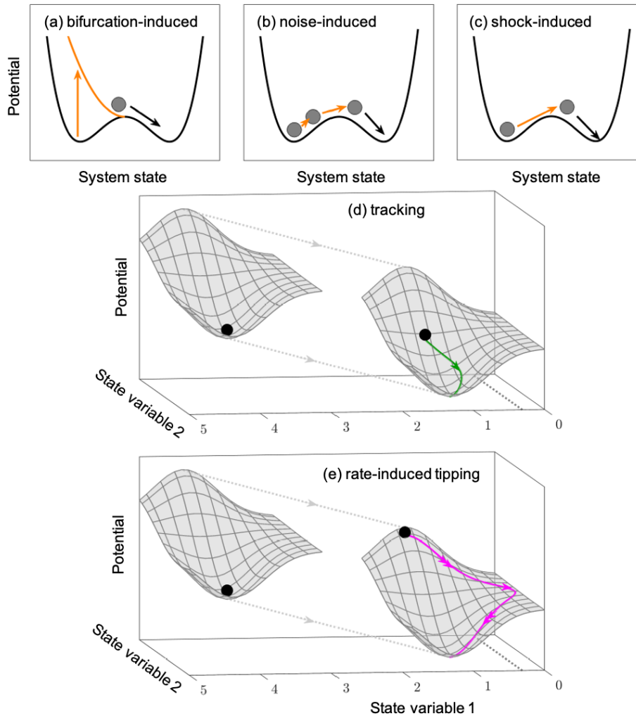
Figure 3. Illustration of the four different tipping mechanisms: (a) bifurcation-induced tipping; (b) noise-induced tipping; (c) shock-induced tipping; and (d, e) rate-induced tipping in the case where no alternative states are present, but the rate-induced tipping refers to a very large excursion in state space with different properties. (d) Rate-induced tipping with a tracking trajectory and (e) rate-induced tipping with a tipping trajectory. For more explanations, see the text.
