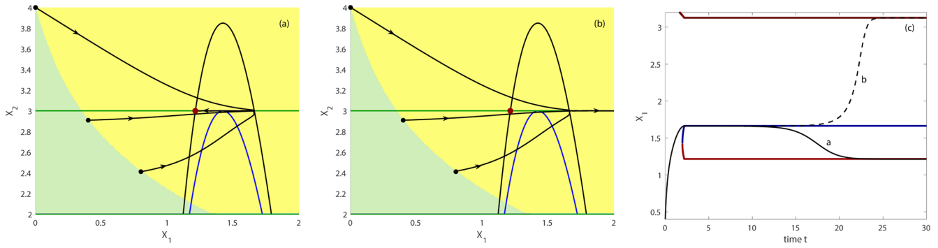
Figure 8. Tipping of trajectories starting next to the non-autonomous basin boundary in the points indicated by small filled black circles; (a) just next to the boundary in the light-green basin and (b) just next to the boundary in the yellow basin. Black nullcline at the critical rate T_r = 2.1698 . In this part of the state space only the light-green and yellow non-autonomous basins are visible. (c) Time evolution of the two trajectories separated by the non-autonomous basin boundary with X_1 = 0.4 at t = 0 (middle trajectory in a and b ).
