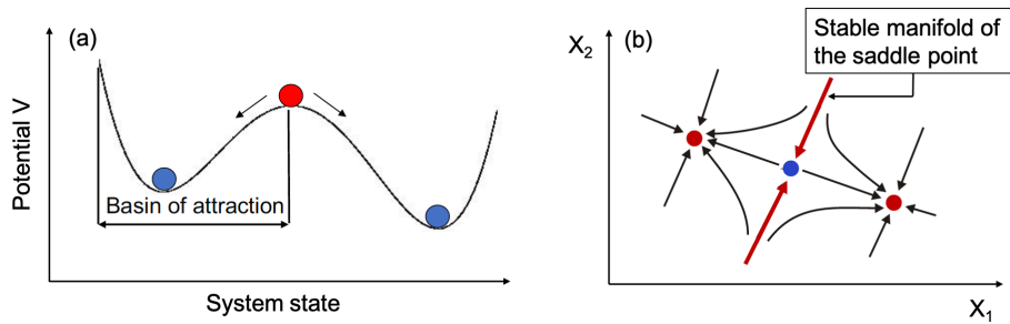
Figure 1. (a) Sketch of the potential (stability landscape) of a bistable system and (b) state space of a bistable system including the unstable saddle point and its stable manifold, which make up the boundary between the two basins of attraction.
