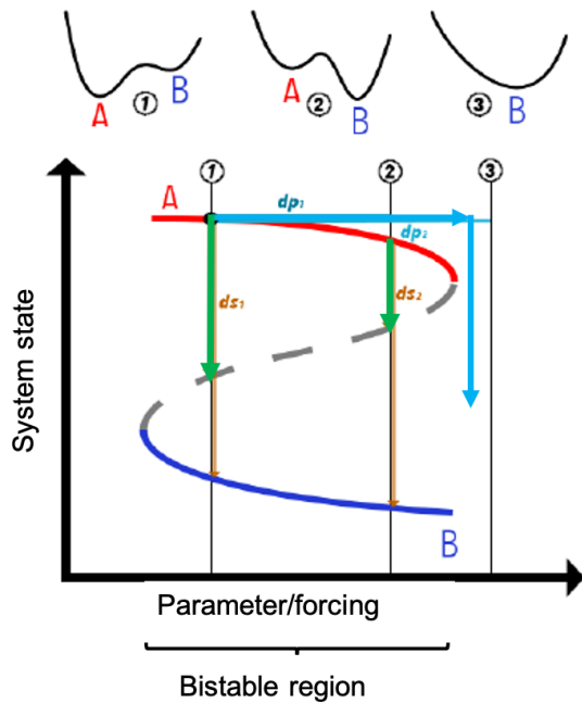
Figure 2. Relationship between the stability landscape and the control parameters/the forcing of the system. Cyan arrows indicate the changes in control parameters or forcings; the light-green and light-brown arrows refer to changes in the state variables.
