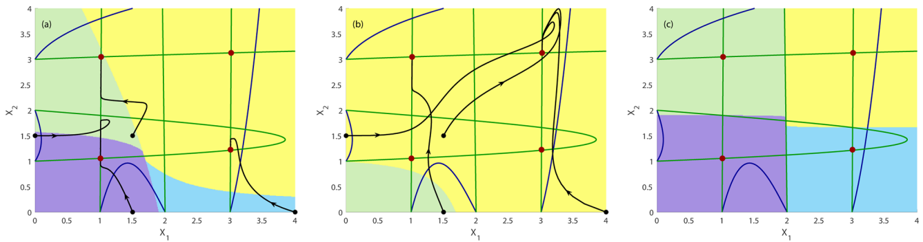
Figure 10. Time evolution of the non-autonomous system shown in Eq. (10) with decreasing impact of the driver c in the interval [0.4, 0.01] together with four exemplary trajectories (timescale separation between system 1 and 2 \varepsilon = 0.1 ): (a) fast rate with 0 \leq t \leq 2.0 , v = -0.15 and T_r = 2.0 and (b) slow rate with 0 \leq t \leq 8.0 , v = -0.0375 and T_r = 8.0 . Attractors are indicated by filled dark-red circles. Dark-blue curves: nullclines at the beginning of the parameter drift at t = 0 and c = 0.4 ; dark-green curves: nullclines at the end of the parameter drift at t = T_{\text{end}} = 200 and c = 0.01 . The non-autonomous basins of attraction are presented at the end of the simulation T_{\text{end}} in light green, yellow, violet and light blue. (c) For comparison: basin of attraction in the frozen-in case for c = 0.01 .
