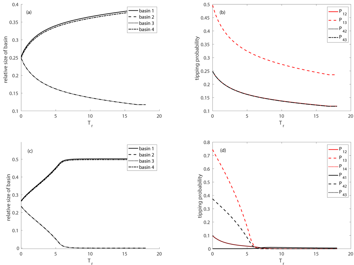
Figure 12. The relative size of the non-autonomous basins of attraction ( a , c ) and tipping probabilities ( b , d ) for the diffusively coupled system shown in Eq. (11) depending on the rate of environmental change measured in terms of T_r ( c_{\text{start}} = 0.4 , c_{\text{end}} = 0.01 ) ( a ) and ( b ) \varepsilon = 1 and ( c ) and ( d ) \varepsilon = 0.1 .
