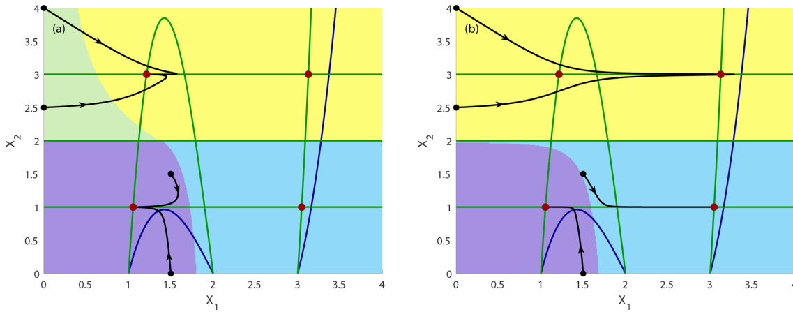
Figure 6. Time evolution of the non-autonomous system shown in Eq. (8) with decreasing impact of the driver c in the interval [0.4, 0.1] together with four exemplary trajectories ( \varepsilon = 1 ): (a) fast rate with 0 \leq t \leq 2.0 , v = -0.15 and T_r = 2.0 and (b) slow rate with 0 \leq t \leq 8.0 , v = -0.0375 and T_r = 8.0 . Attractors are indicated by filled dark-red circles. Dark-blue curves: nullclines at the beginning of the parameter drift at t = 0 and c = 0.4 ; dark-green curves: nullclines at the end of the parameter drift at t = T_{\text{end}} = 200 and c = 0.1 . The non-autonomous basins of attraction are presented at the end of the simulation T_{\text{end}} in light green, yellow, violet and light blue.
