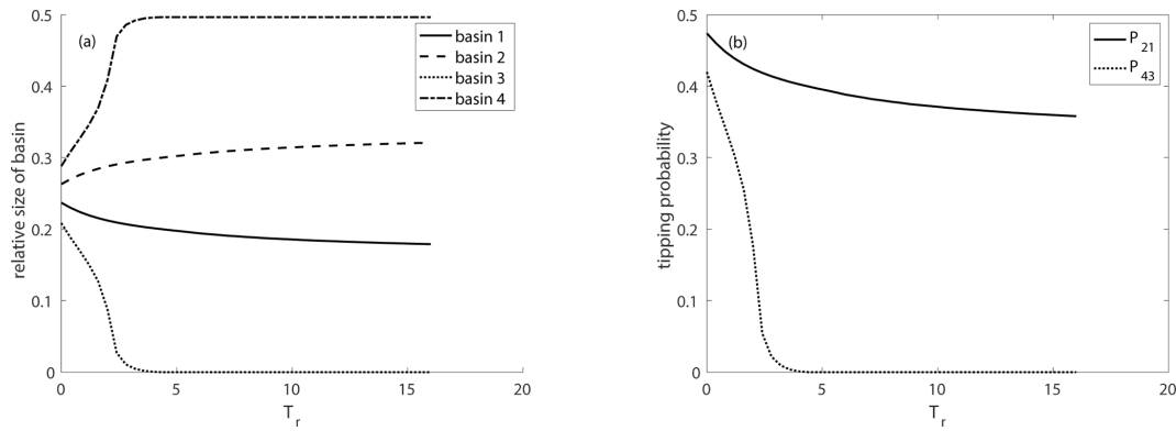
Figure 7. The relative size of the non-autonomous basins of attraction (a) and tipping probabilities (b) for the drive–response coupled system shown in Eq. (8) depending on the rate of environmental change measured in T_r , \varepsilon = 1 , c_{\text{start}} = 0.4 and c_{\text{end}} = 0.1 .
