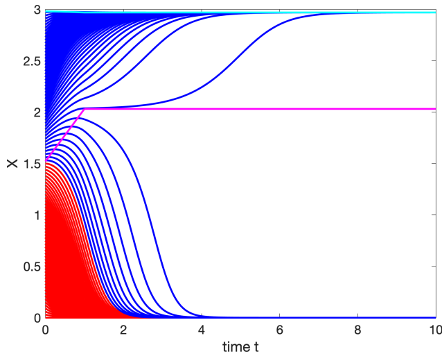
Figure 4. Time evolution of trajectories of system Eq. (4) with parameter drift in b with 1.5 \leq b \leq 2 . The movement of the saddle point X^{(2)} demarking the basin boundary is shown in magenta, while the movement of the stable state X^{(3)} is shown in cyan. All trajectories colored red would have converged to the extinction state X^{(1)} in the frozen-in case b = 1.5 , while blue trajectories would have converged to the high population state X^{(3)} . Parameters: r = 2.0 , K = 3.0 , m = 0.02 , v = 0.5 and T_r = 1.0 .
