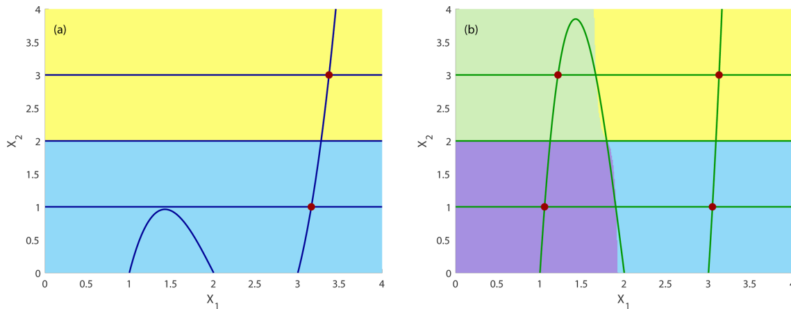
Figure 5. Basins of attraction, attractors and nullclines for the autonomous system shown in Eq. (7) with fixed coupling for two different constant coupling strengths c (frozen-in case) and no timescale separation between system 1 and 2 ( \varepsilon = 1 ): (a) c = 0.4 and (b) c = 0.1 . Attractors are indicated by a filled dark-red circle. Dark-blue curves: nullclines \dot{X}_1 = 0 and \dot{X}_2 = 0 at c = 0.4 ; dark-green curves: nullclines \dot{X}_1 = 0 and \dot{X}_2 = 0 at c = 0.1 . The basins of attraction of the four attractors are plotted in light green, yellow, violet and light blue.
