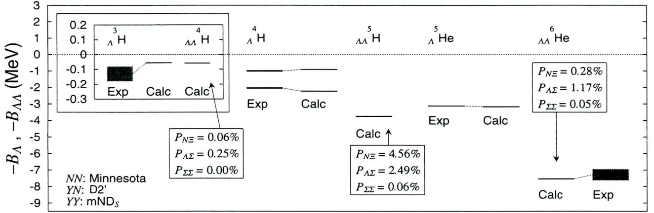
FIG. 1. \Lambda and \Lambda\Lambda separation energies of A = 3 - 6 , S = -1 and -2 s -shell hypernuclei. The Minnesota NN , D2' YN , and mND_5 YY potentials are used. The width of the line for the experimental B_\Lambda or B_{\Lambda\Lambda} value indicates the experimental error bar. The probabilities of the N\Xi , \Lambda\Sigma , and \Sigma\Sigma components are also shown for the \Lambda\Lambda hypernuclei.
