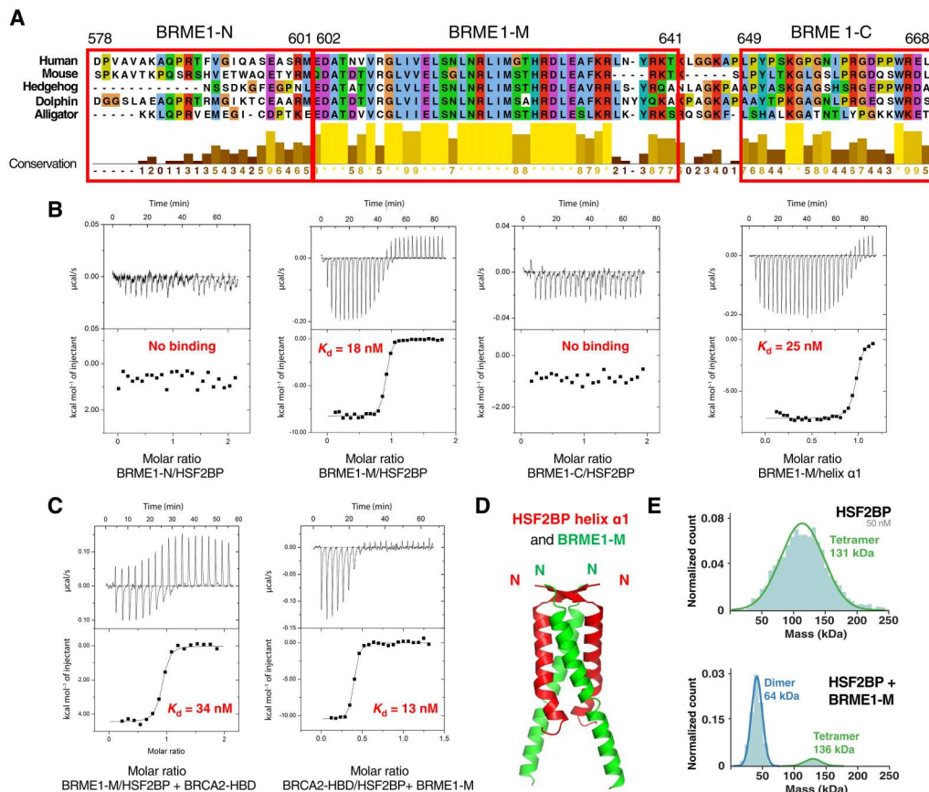
Fig. 4. A BRME1 peptide binds to helix α1 and disrupts the HSF2BP tetramer. (A) Sequence alignment of the C-terminal region of a set of five BRME1 proteins, showing a representative sequence diversity. The sequences corresponding to the three human peptides BRME1-N, BRME1-M, and BRME1-C are boxed. (B) ITC curves identifying the BRME1 sequence binding to HSF2BP. These experiments were all performed at 30°C. Additional experiments performed at 20°C are detailed in fig. S5A and Table 1. (C) ITC curve showing that BRME1-M and BRCA2-HBD do not compete for binding to HSF2BP. These experiments were performed at 20°C. (D) Crystal structure of the HSF2BP peptide E19-V50 (helix α1, in red) bound to the BRME1 peptide E602-K641 (BRME1-M, in green). Each asymmetric unit contained a HSF2BP-BRME1 dimer. The heterotetramer was calculated by application of a twofold crystallography symmetry (table S2). (E) Mass photometry experiment performed on either free HSF2BP (top) or HSF2BP bound to BRME1-M (bottom). The distribution of masses is displayed for samples at a concentration of 50 nM for HSF2BP and 100 nM for BRME1-M. HSF2BP analyzed at 25 nM is shown in fig. S6C.
