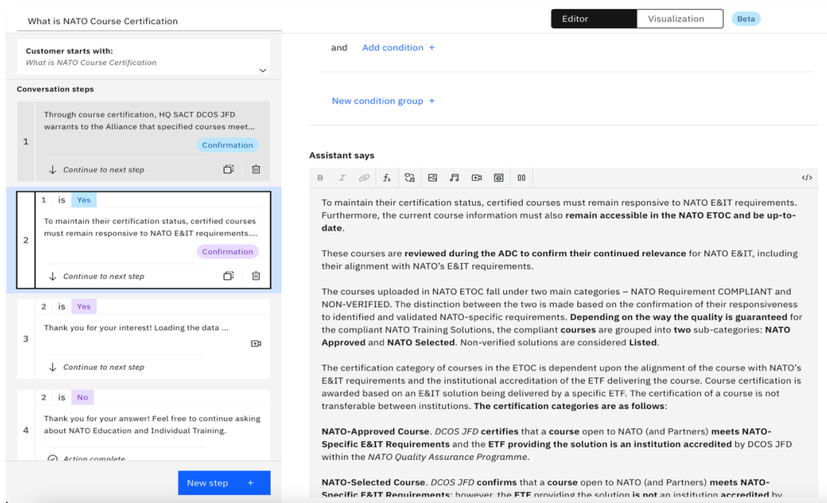
Fig. 11 - IBM Watsonx Assistant admin interface view for content creation
