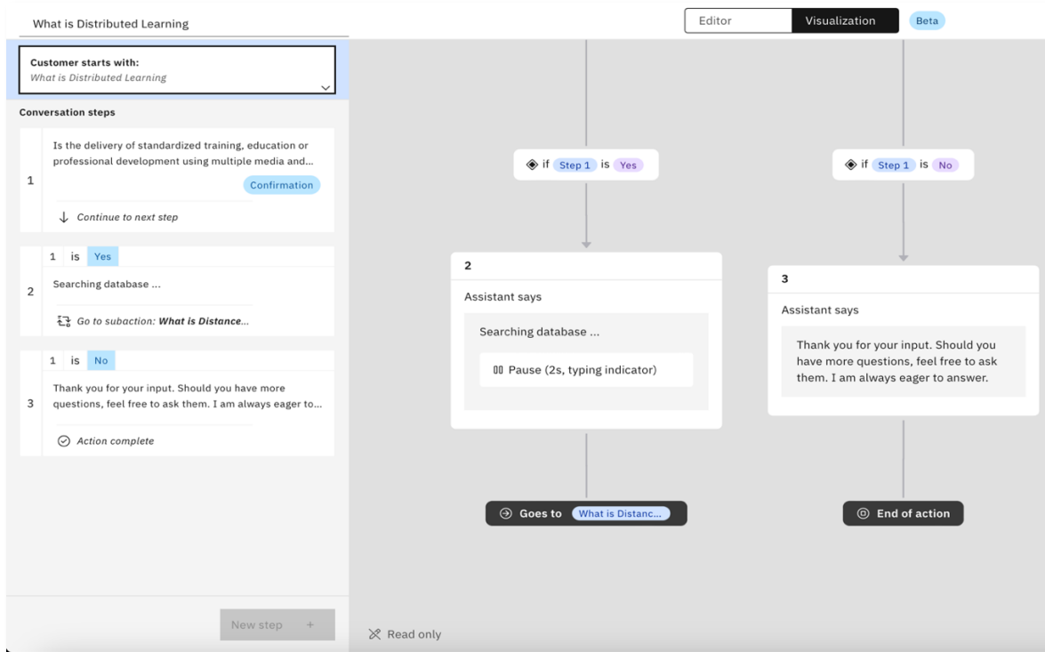
Fig. 12 - IBM Watsonx Assistant admin interface view for dialog logic flow
