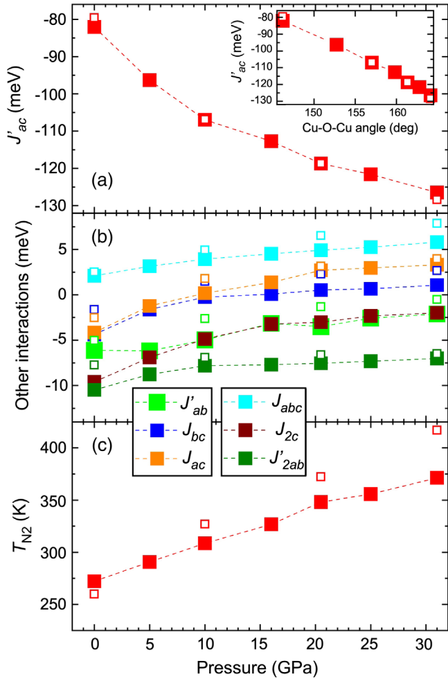
FIG. 4. Pressure dependence of (a) J'_{ac} , (b) J'_{ab} , J_{bc} , J_{ac} , J_{abc} , J_{2c} , and J'_{2ab} , and (c) T_{N2} . Closed and open symbols show the results of the LMTO and QE calculations, respectively. The notations for the parameters are shown in Fig. 3. The inset in (a) shows the dependence of J'_{ac} on the angle Cu-O-Cu.
