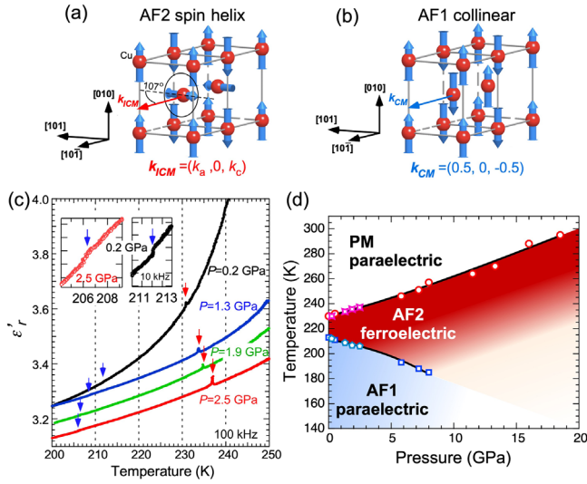
FIG. 1. Schematics of (a) spin-helix structure with incommensurate \mathbf{k}_{\text{ICM}} = (k_a, 0, k_c) in the AF2 phase (the angle between \mathbf{k}_{\text{ICM}} and the spiral plane is \sim 107^\circ ), and (b) collinear structure with commensurate \mathbf{k} = (0.5, 0, -0.5) in the AF1 phase. (c) Pressure dependence of the real part of the relative dielectric permittivity of CuO. Inset: expansion around lower phase transition temperature T_{N1} at 0.2 GPa and 2.5 GPa. (d) Temperature versus pressure phase diagram of multiferroic CuO. Square (circle) and pentagon (star) symbols denote phase transition temperature points of T_{N1} ( T_{N2} ) determined by neutron diffraction and dielectric permittivity experiments, respectively.
