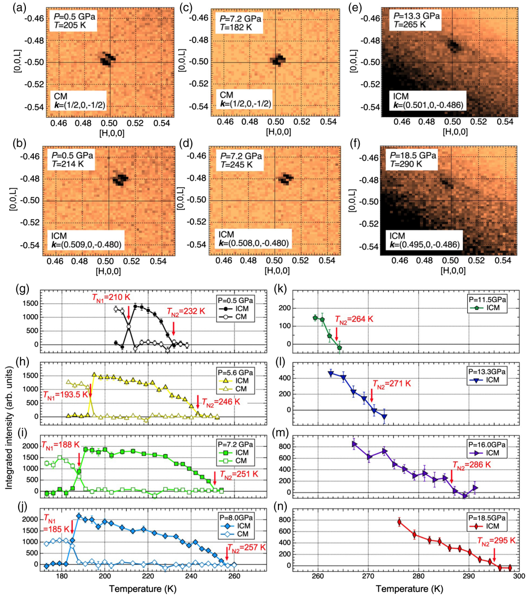
FIG. 2. (a)–(f) Neutron diffraction intensity maps near reciprocal lattice position, \mathbf{Q} = (0.5, 0, -0.5) in the (H, 0, L) plane, measured at typical pressures and temperatures. (g)–(n) Plots depict integrated intensities of magnetic Bragg reflections associated with commensurate \mathbf{k} = (0.5, 0, -0.5) (open symbol) and incommensurate \mathbf{k} = (k_a, 0, k_c) magnetic phases for typical pressures and temperatures.
