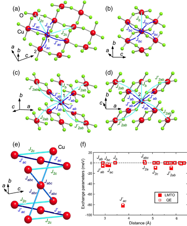
FIG. 3. Superexchange interaction paths (a) in the ac plane, (b) the bc plane, and (c),(d) in the ab plane around Cu sites 1 and 2. (e) Long-range interactions J_{abc} between the ac planes. (f) Distance dependence of isotropic superexchange interactions, as obtained in the QE and LMTO methods at ambient pressure.
