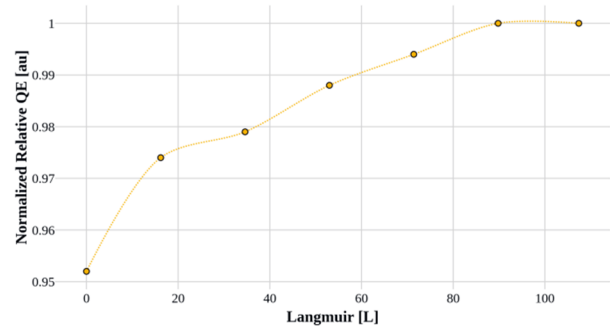
Figure 2: Normalized relative QE of an O 2 degraded Ag polycrystalline cathode as a function of CO exposure.
