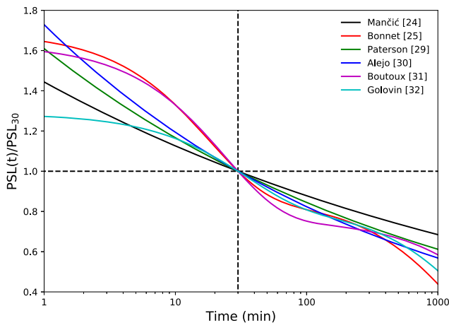
FIG. 1. Comparison of different fading functions from Mančić et al. , 24 Bonnet et al. , 25 Paterson et al. , 29 Alejo et al. , 30 Boutoux et al. , 31 and Golovin et al. 32 The functions given by each group have been converted into the formula for PSL(t)/PSL_{30} for consistency with the chosen convention for this work and to aid comparisons.
