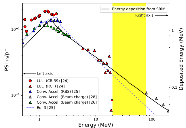
FIG. 2. Left axis: Comparison of the experimentally measured responses (converted to PSL_{30} per proton using the fading functions and times specified in each work) by Mančić et al. , 24 Bonnet et al. , 25 Rabhi et al. , 28 and Freeman et al. 26 The legend indicates the proton source for each dataset as well as the method used to determine the proton number incident on the IPs (in brackets). The yellow region represents the energy range in which no calibration data have been reported. The blue dashed line represents the response curve given by Eq. (3), as determined by Bonnet et al. , 25 using values for their reported parameters. 35 Right axis: Energy deposited by protons in the active layer, E_{Dep} , obtained from SRIM simulations 36,37 (black line). A peak in the energy deposition is observed at \sim 1.6 MeV.
