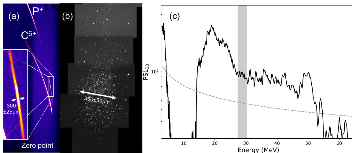
FIG. 5. (a) Scanned IP image converted to PSL with each trace corresponding to ions with specific q/m labeled. The inset shows a zoomed in portion of the proton trace, which was measured to be (300 \pm 25) \mu\text{m} wide. Behind the IP was a 1250 \mu\text{m} Cu filter and CR-39. (b) Microscopic image of the proton pits on the front surface of CR-39 after etching at \times 20 magnification. The width of the pit streak was measured to be \sim (350 \pm 50) \mu\text{m} . (c) Background subtracted PSL_{30} profile across the proton trace in the IP shown in (a). The shaded region indicates the energy range, which the CR-39 detected protons. The detection limit of the IP is shown as the dashed gray line.
