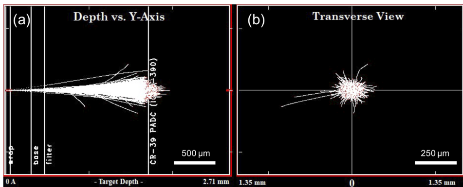
FIG. 4. Outputs from SRIM simulation of the detector assembly in Fig. 3(d) using the 1250 \mu\text{m} Cu filter and 27.4 MeV incident proton energy, corresponding to the data shown in Fig. 5(a). Scale bars are shown in the bottom right corners. (a) Trajectories of 27.4 MeV protons in the Y-Z plane (Z is the direction of travel). (b) Transverse (X-Y) distribution of the protons on the CR-39 front surface, where the lateral straggle of the protons is calculated as \sim 70 \mu\text{m} .
