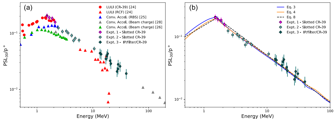
FIG. 6. (a) The calculated IP response data from the experiments described in this work, as labeled in Table I, compared to the experimental data reported by previous studies as shown in Fig. 2. Vertical error bars represent an error of ~10%–15% in counting the pits in CR-39 and determining the energy range over which to integrate the PSL. The errors for data from the slotted CR-39 were smaller, as the PSL in each energy bin could be determined more precisely. Horizontal errors are small but arise from the width of the energy bins calculated from the CR-39 bins for the high energy data, and for the low energy data using the slotted CR-39 grid, they were determined by the resolution of the TPS. (b) The same experimental data as in (a) fit using two different models from Eqs. (3) and (4) with newly determined values of the sensitivity parameter, \alpha , and quenching factor, kB , via a least squares fitting. The dashed black line represents the best fit function described by Eq. (8).
