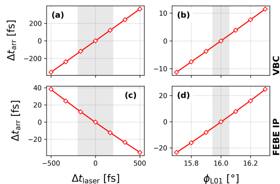
Figure 4: Change in the bunch arrival time at the VBC (top) and FEBE IP (bottom), plotted as functions of the PI laser timing jitter (left) and linac 1 phase jitter (right).
