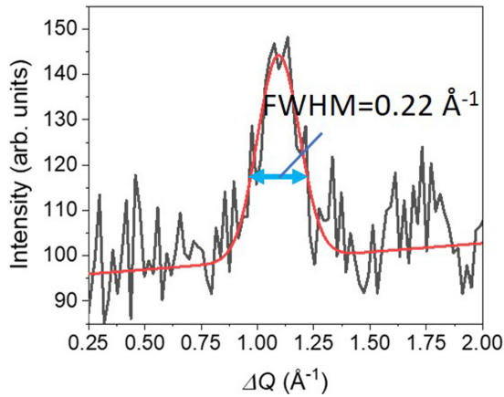
FIG. 5. An intensity trace (black line) across an R -type reflection in Fig. 4. The red line corresponds to a Gaussian fitted to this trace. A full width at half maximum (FWHM) is indicated. The spherical domain size D can be estimated according to the Scherrer's formula as D = 6.96/(\text{FWHM}) \approx 3.2 nm.
