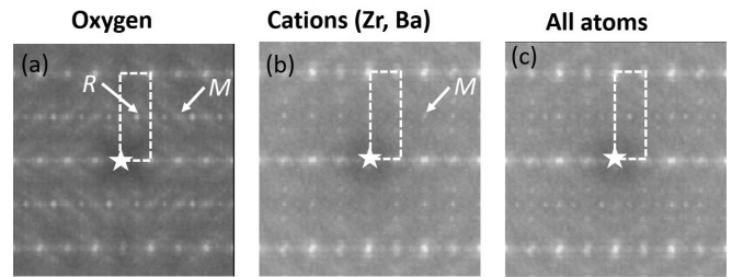
FIG. 11. The \{310\} sections of reciprocal space with calculated x-ray diffuse scattering for a refined configuration of BaZrO 3 at 2 K using (a) oxygen atoms, (b) Zr and Ba, (c) all species. The R spots apparently arise exclusively from oxygen whereas the M -spot intensities are dominated by the cations with small contributions from oxygen.
