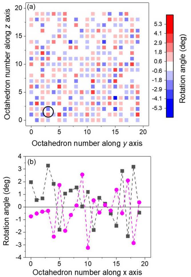
FIG. 9. (a) A representative \{yz\} layer of the refined configuration for BaZrO 3 at 2 K. Squares symbolize [\text{ZrO}_6] octahedra with the color scale encoding their rotation angles around the x axis. The blue and red colors correspond to the negative and positive signs of rotations, respectively. The presence of extended regions with chessboard patterns of positive and negative rotations is evident. (b) Rotation angle as a function of the octahedron’s number along the two adjacent octahedral chains [encircled in (a)] parallel to the x axis. The rotations in the two neighboring chains occur preferentially out of phase with each other, which indicates that the in-plane order of rotations is maintained in multiple \{yz\} layers. Segments with in-phase tilting along the octahedral chains are observed as well.
