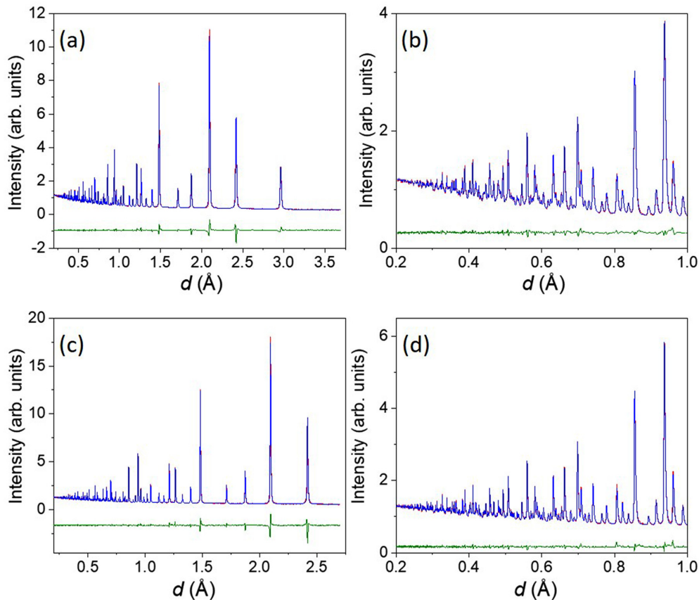
FIG. 2. Experimental (red) and calculated (blue) neutron diffraction patterns for \text{BaZrO}_3 at 2 K for the (a,b) 90^\circ and (c,d) 146^\circ detector banks. The calculated signals correspond to the structural model obtained using Rietveld refinements in GSAS. The difference traces are shown in green.
