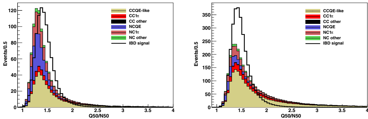
FIG. 14. The q_{50}/n_{50} distributions for the atmospheric neutrino and IBD Monte-Carlo simulations, for events with E_{\text{rec}} \in [7.5, 29.5] MeV (left) and E_{\text{rec}} \in [15.5, 79.5] MeV (right). We consider only events reconstructed in the FV and passing the noise reduction cuts. The assumed DSNB spectrum is taken from the Horiuchi + 09 6 MeV model [16]. The signal and background distributions are normalized to the same area.
