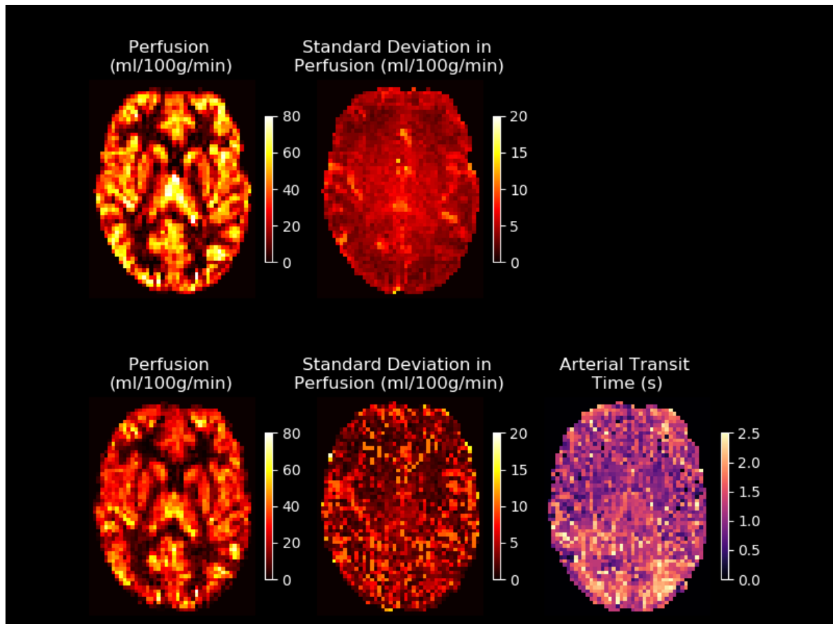
Figure 1: Example quantified perfusion images from single-delay (top row) and multi-delay (bottom row) ASL in a single subject. Also shown are the estimated uncertainty in the perfusion parameter, given as the estimated standard deviation on the perfusion value in the voxel, and the corresponding ATT estimates for the multi-delay data. The single-delay data has been fitted in “white paper” mode, following the assumptions of the ASL consensus paper. Due in particular to the assumption that ATT = 0 s, the resultant perfusion estimates are higher than in the multi-delay case. In the multi-delay case, fitting an extra parameter (ATT) increases the uncertainty in perfusion estimates for some voxels, leading to a more variable standard deviation map for this parameter.
