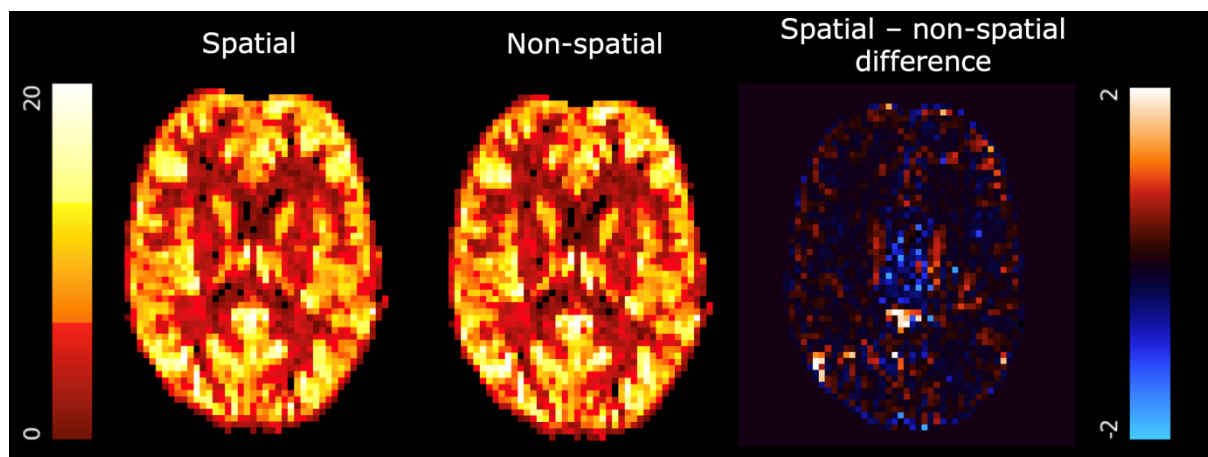
Figure 4. Perfusion maps derived from single-delay pseudo-continuous ASL with (left) and without (centre) spatial regularisation. The difference image is shown on the right. Quantities are in arbitrary units (i.e., non-calibrated data)
