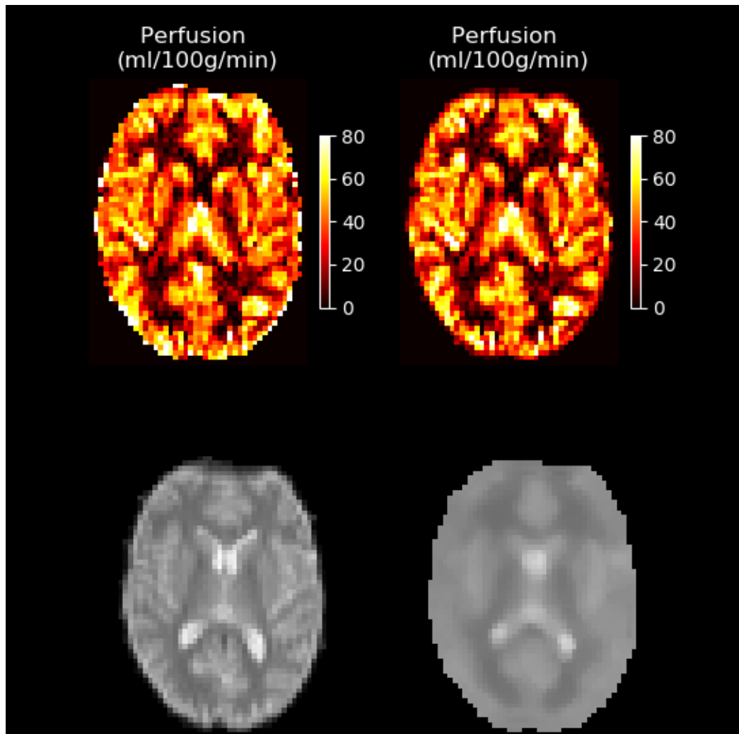
Figure 5: Calibration using a voxelwise approach. Left: calibration using the original calibration image (lower image) results in spurious high perfusion voxels around the pial boundary of the brain. Right: Pre-processing of the calibration image (lower image) reduces the presence of CSF in pial voxels of this image, which suppresses artefacts in the resulting perfusion image.
