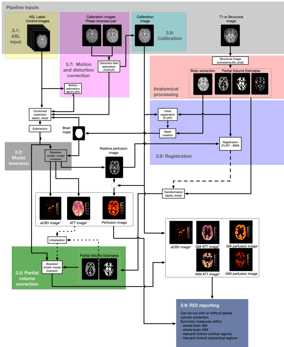
Figure 3: A graphical representation of the processing steps required to produce a perfusion image (scaled into absolute units) along with ATT. The numbers 3.1, 3.2 etc refer to section headings in the manuscript text. Optional steps such as motion/distortion correction and partial volume correction have been included. * denotes an output for which multi-delay data is required
