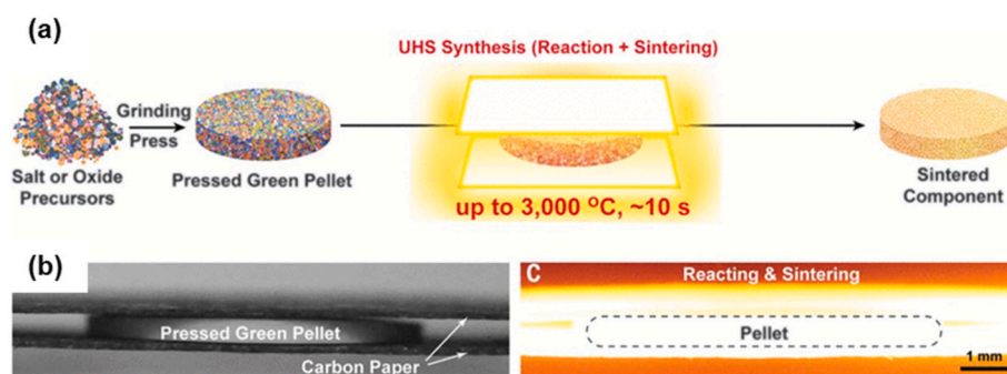
Fig. 8. (a) Schematic of the UHS synthesis process, (b) Photographs of the UHS sintering setup at room temperature without applying current, and (c) at \sim 1500\text{ }^{\circ}\text{C} [205].
