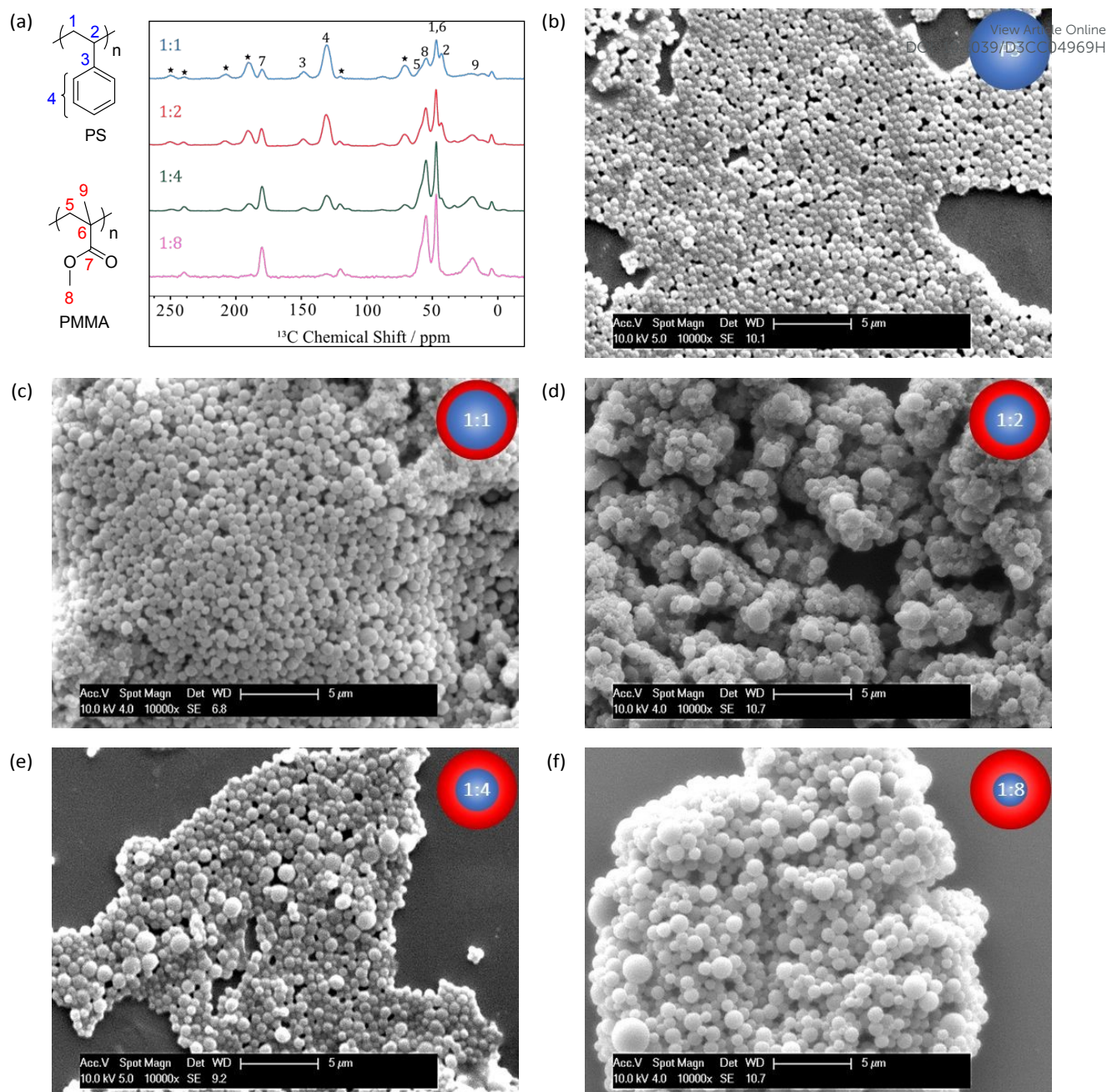
Figure 2: (a) ^1\text{H} - ^{13}\text{C} CP-MAS spectra of PS-PMMA core-shell polymers with PS:PMMA ratios of 1:1, 1:2, 1:4 and 1:8 (note: spinning sidebands marked with \star , inset shows numbering of ^{13}\text{C} assignments), and SEM micrographs of (b) PS particles (core), and PS-PMMA core-shell particles with targeted mass ratios of (c) 1:1, (d) 1:2, (e) 1:4 and (f) 1:8.
