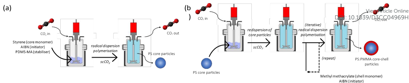
Figure 1: Reaction schematic of (a) PS core and (b) PMMA shell syntheses in supercritical CO 2 in a high-pressure autoclave
