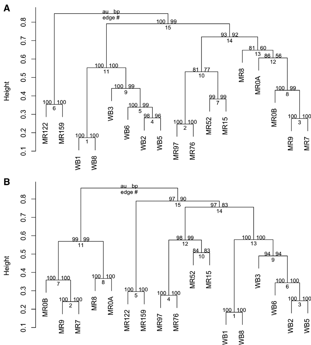
Fig. 8. Hierarchical clustering of bacterial communities sampled at study sites on 26 September using Jaccard distance (A) and bray-Curtis dissimilarity (B) matrices and average-linkage (UPGMA) clustering methods. Values above nodes reflect cluster uncertainty based on approximately unbiased p -values (au; left) and bootstrap probability (bp; right) generated via resampling ( n = 10,000).
