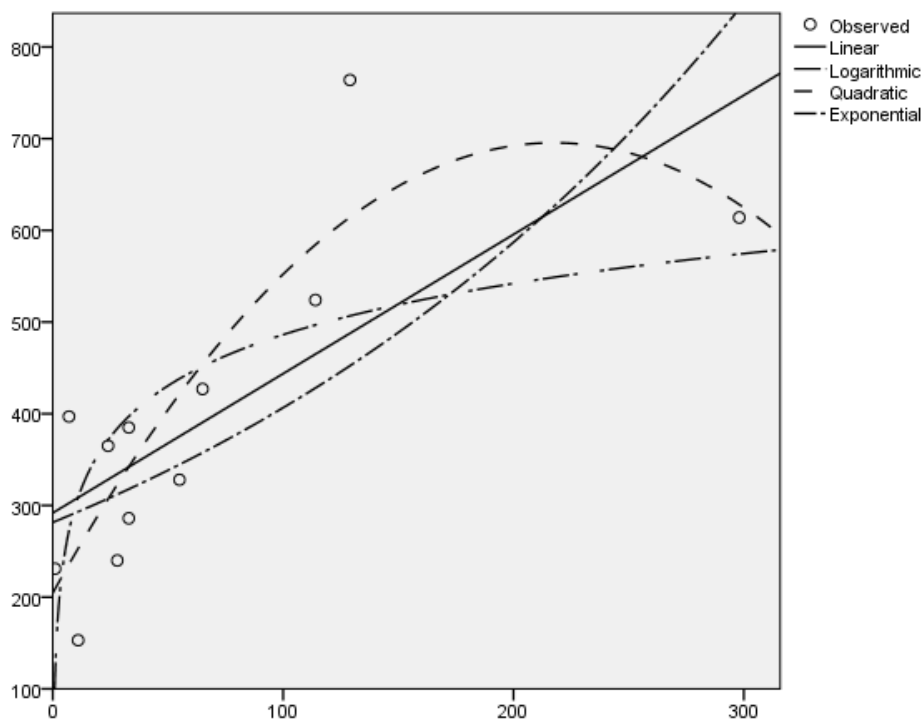
Figure 4. Comparison plot of the relationship between inflation and economic growth with the modeling carried out
