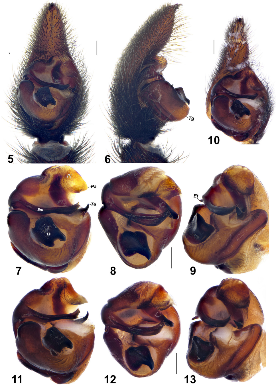
Figures 5–13. Palps and bulbs of Acantholycosa voronii sp. nov. (5–9) and A. irinae (10–13): 5, 10 – palps, ventral; 6 – ditto, prolateral; 7, 11 – bulbs, ventral; 8, 12 – ditto, anterior; 9, 13 – ditto, retrolateral. Abbreviations: Em – embolus, Et – embolic tooth, Pa – paleal apophysis, Pl – palea, Ta – tegular apophysis, Te – terminal apophysis, Tg – tegulum. Scale bars: 0.2 mm.
