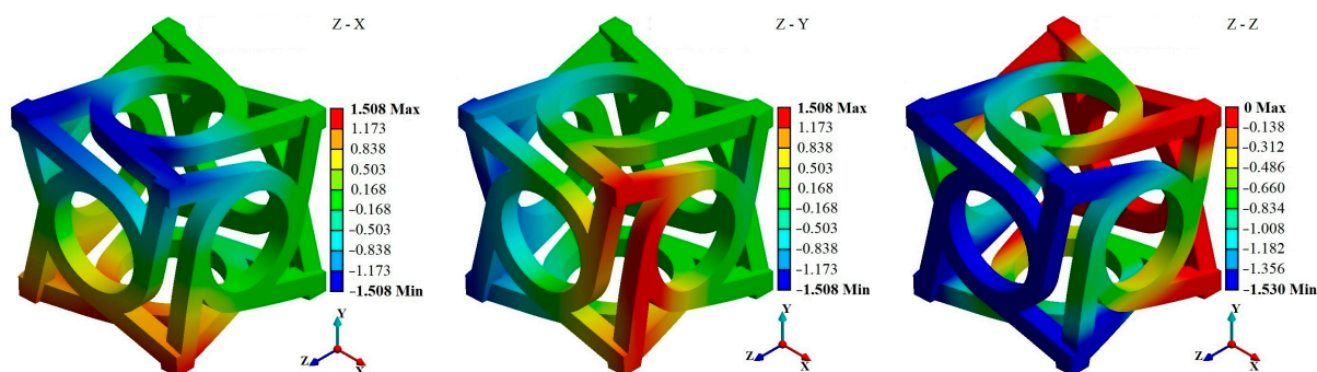
Figure 4. Mechanical behavior of the pattern A unit cell loaded along three orthogonal axes.
