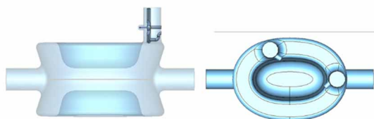
Figure 13: Coaxial damping with ILC type couplers.
