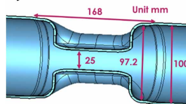
Figure 15: The bare 1.3 GHz WOW crab cavity.
