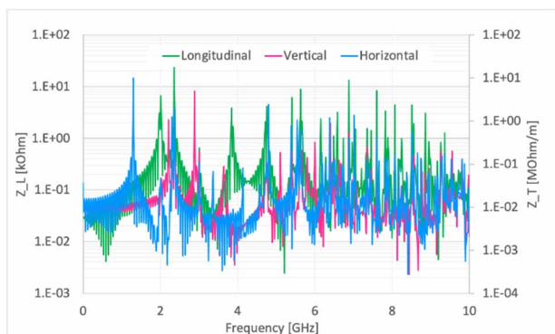
Figure 12: Impedance spectrum of the DQW bare cavity.
