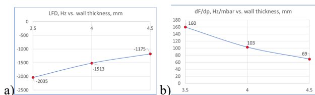
Figure 20: a) Calculated LFD coefficients and b) dF/dP of QMiR cavity with different wall thicknesses.
