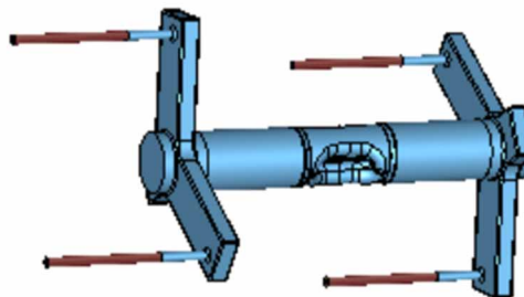
Figure 16: Cu waveguide-coax damper for WOW cavity.
