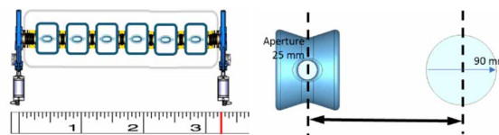
Figure 14: Preliminary integration in a cryomodule (left) and the cavity to adjacent beam pipe separation (right).
