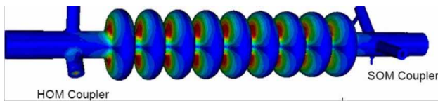
Figure 2: The original elliptical 3.9 GHz crab cavity developed for the ILC TDR.
