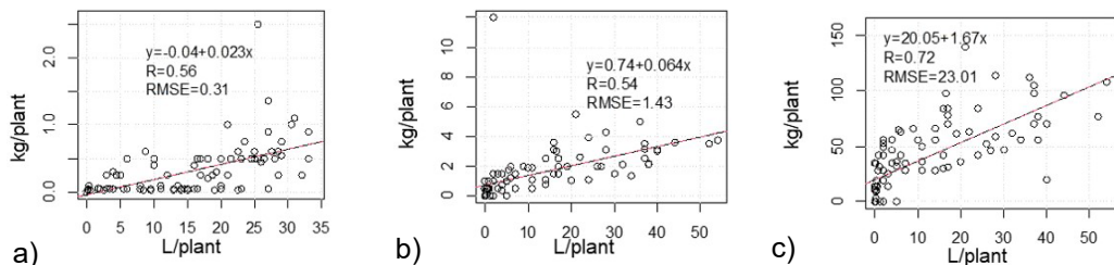
Figure 2. Regression and correlation: a) Y-2020 and FDW-2020; b) Y-2021 and FDW-2021, and c) Y-2021 and FDV-2021.
