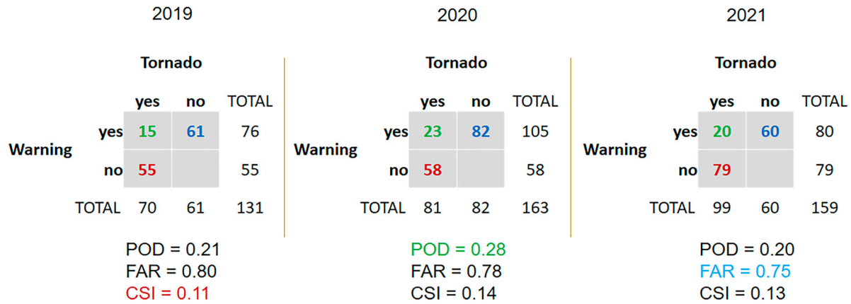
Fig. 3 Contingency tables for 2019 (left), 2020 (centre) and 2021 (right) showing hits (green), misses (red), false alarms (blue) and column and row totals. POD, FAR and CSI calculations for each year are also shown. We note some of the extremes here – the CSI was lowest in 2019 (red), the POD highest in 2020 (green) and the FAR lowest in 2021 (blue).
