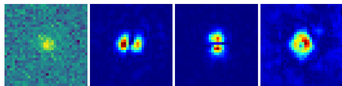
Fig. 10. Saliency map of ASID-FE's features prediction for a single source. The images are from left to right: original image, saliency for x , saliency for y , and saliency for flux . The colour map indicates the degree of importance assigned to each pixel in the image. The brighter the colour, the more important the pixel is for the prediction. As expected, the network mainly focuses on the source to determine its centre and flux while paying less attention to the edges of the image.
