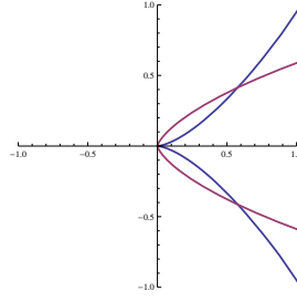
The involute of the 3/2 cusp at 0. Figure 3.
