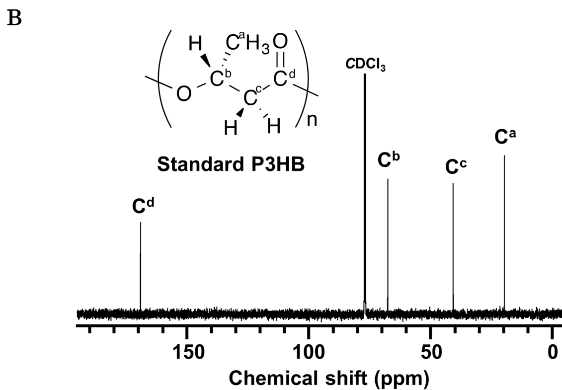
Figure S6: (A) 1 H and (B) 13 C NMR spectra of standard PHB.
