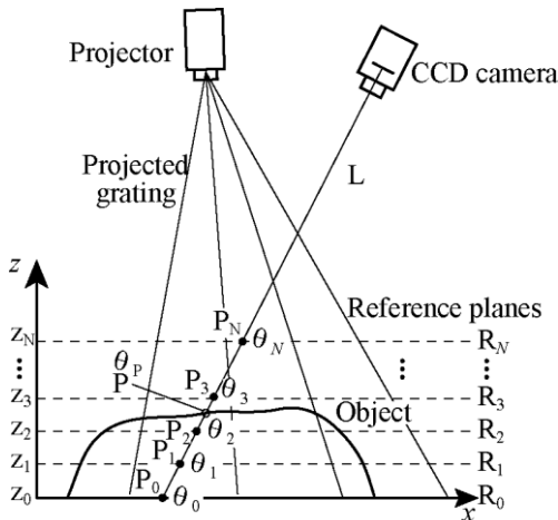
Fig. 1 Principle of the calibration method using whole-space tabulation
