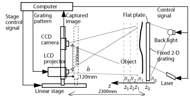
Fig. 3 Optical setup
