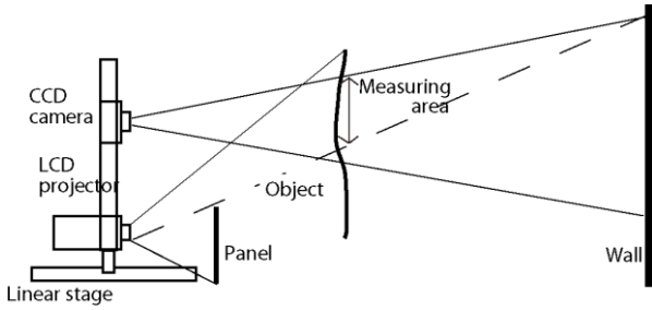
Fig. 4 Panel setting for measurement of translucent object
