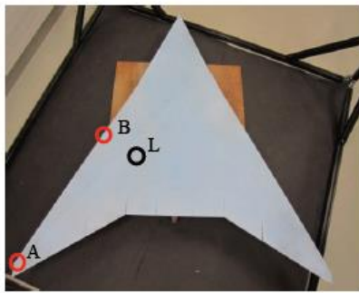
L : LOADING POINT A,B : MEASURED POINTS BY VERNIER CALIPER CORD LENGTH: 1390mm WING SPAN: 1610mm
