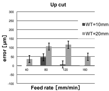
Fig. 6 Measured machining error (Up cut)
